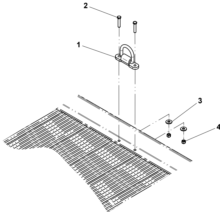
ALUMINUM DECK
