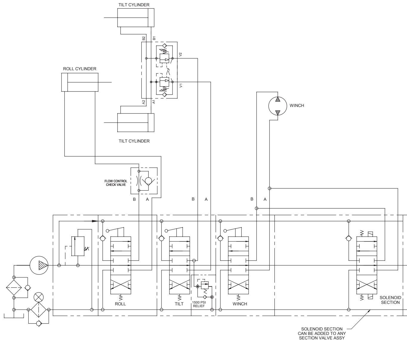
4 Bank Control Valve - Stabilizer with Tow
