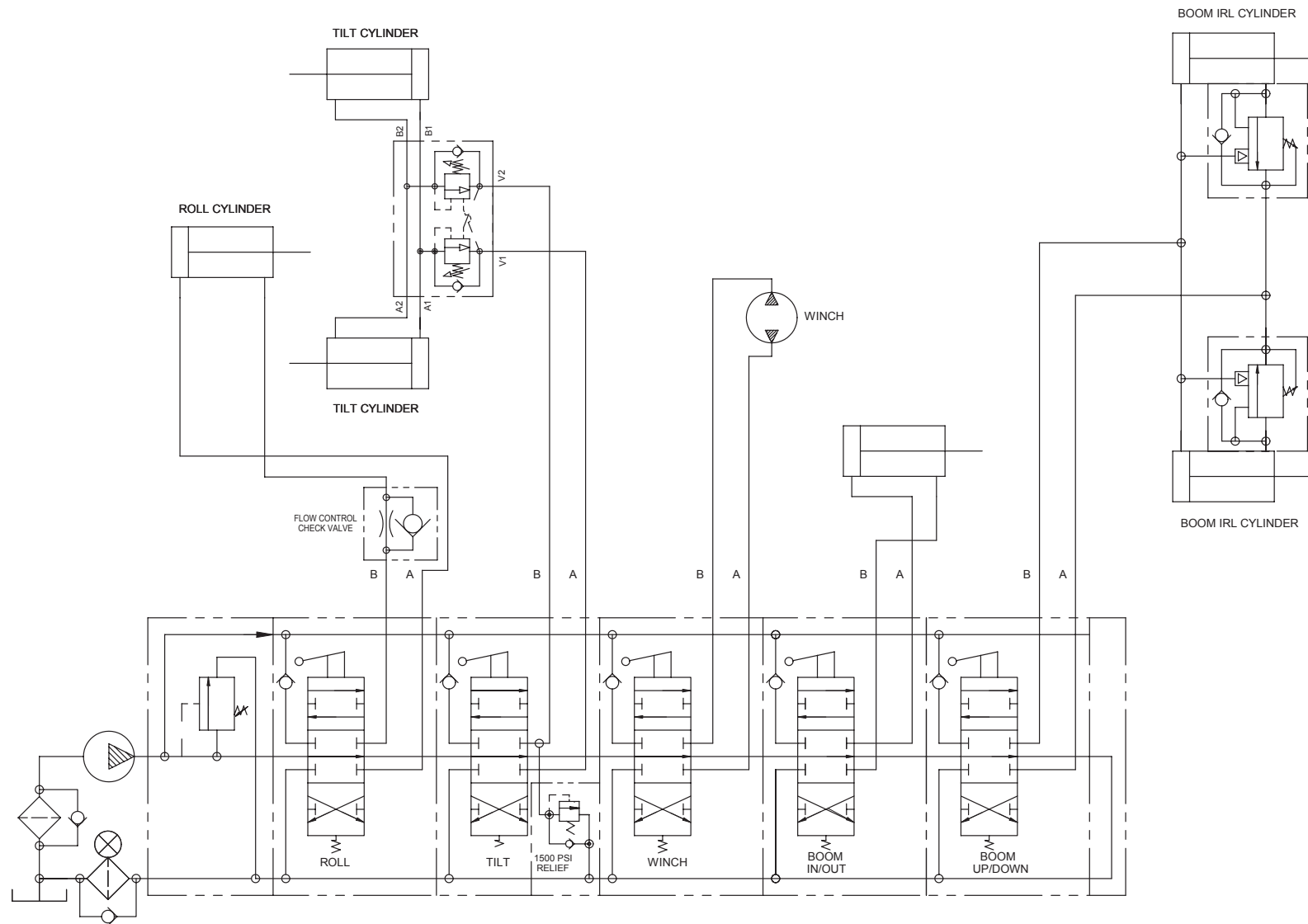
5 Bank Control Valve - IRL Tow Options
