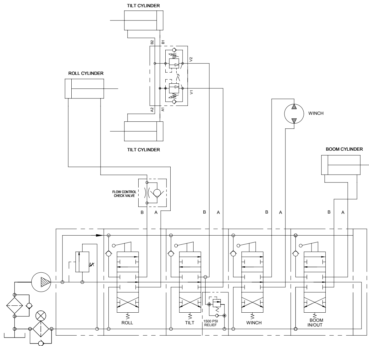
6 Bank Control Valve - ZOD Tow Option
