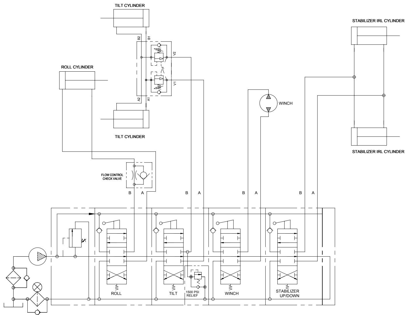
4 Bank Control Valve - Hydraulic Extended Boom Tow Options
