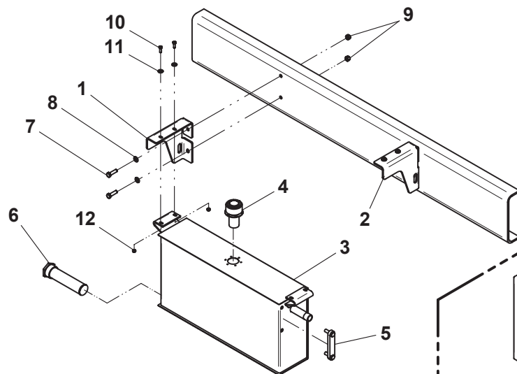
HYDRAULIC TANK ONLY
