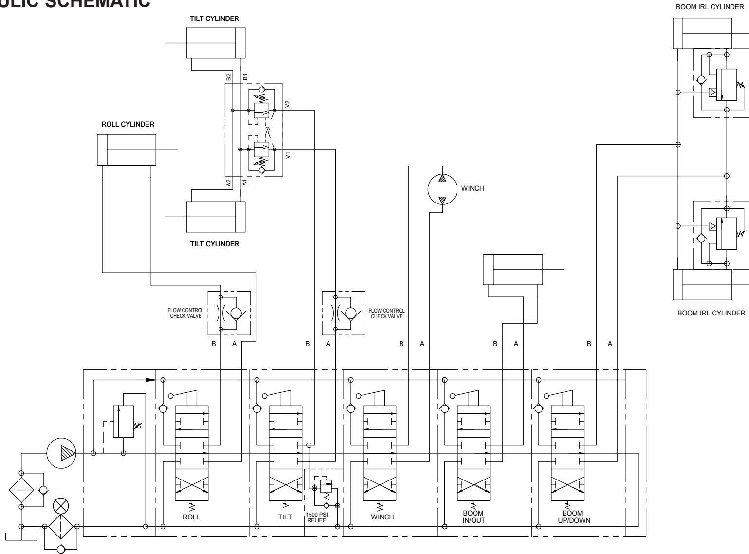
5 Bank Control Valve - IRL Tow Options
