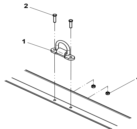
STEEL DECK
