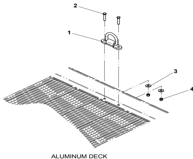
ALUMINUM DECK
