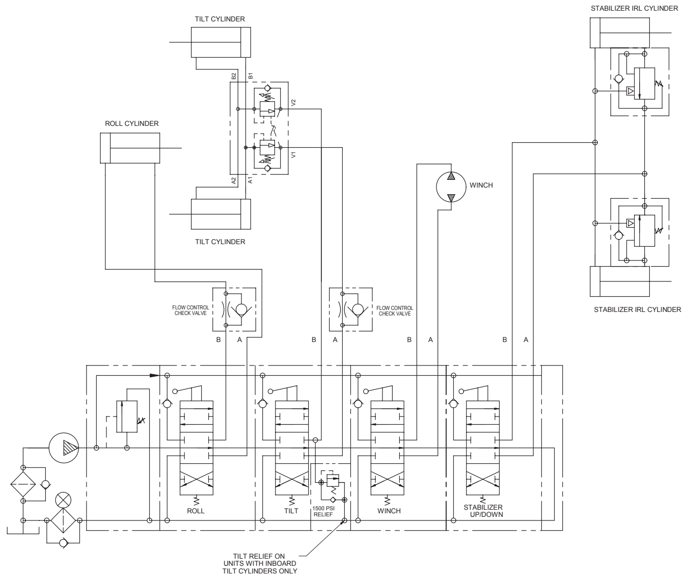
4 Bank Control Valve - Stabilizer with Tow Options
