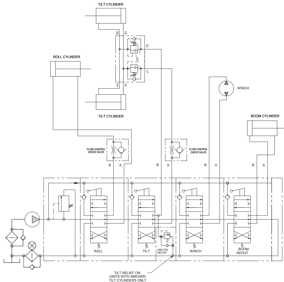
4 Bank Control Valve - Hydraulic Extended Boom Tow Options
