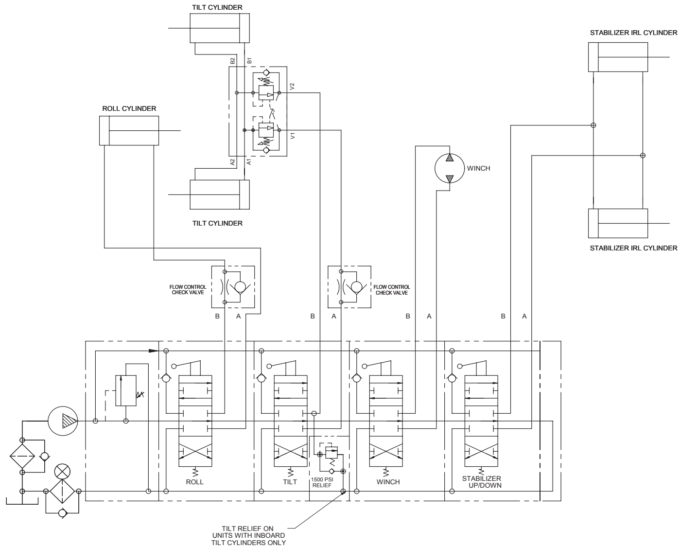
4 Bank Control Valve - Stabilizer Option
