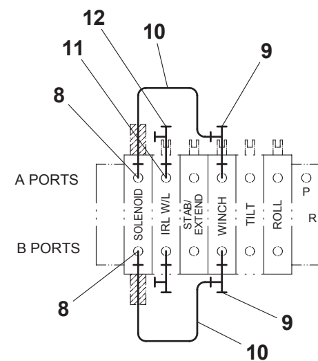
HYDRAULIC SYSTEM COMPONENTS
