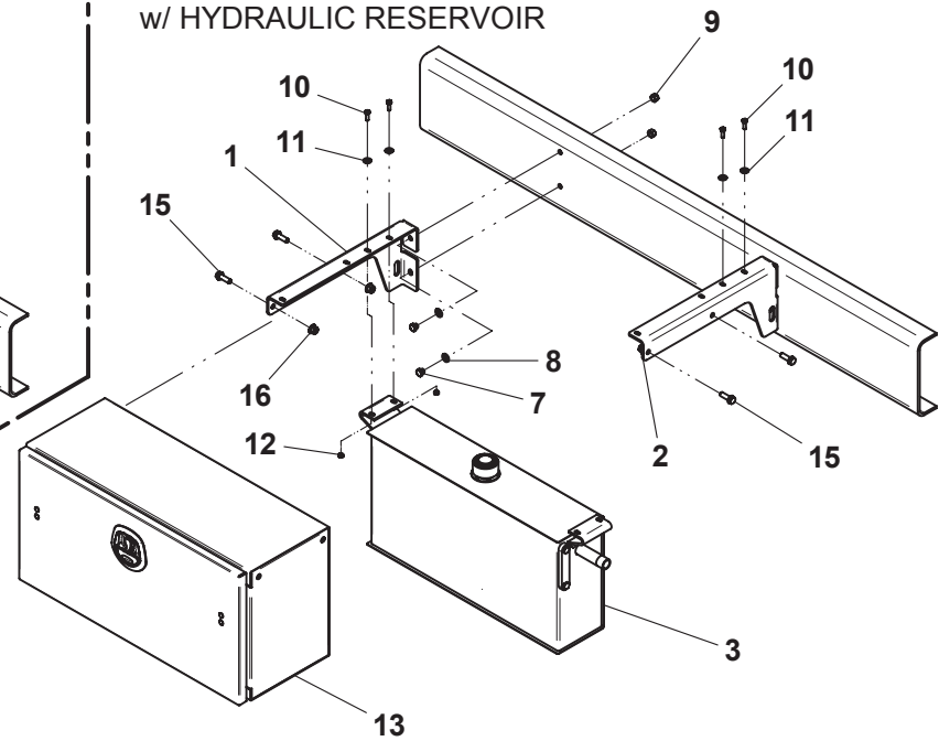
36" TOOLBOX w/ HYDRAULIC RESERVOIR
