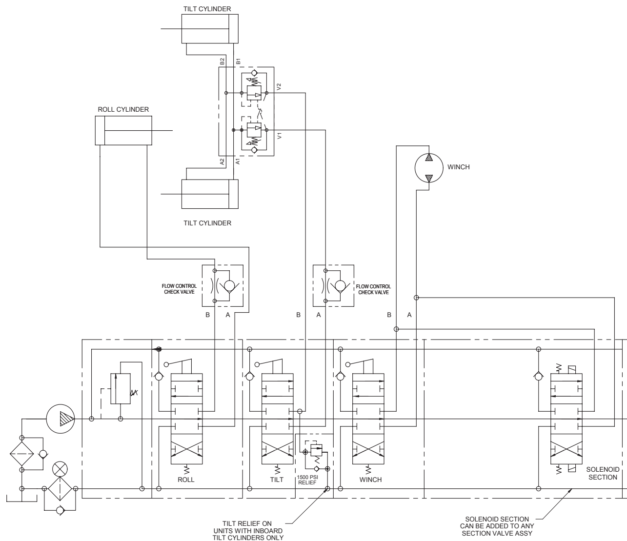
3 + 1 Bank Control Valve - Solenoid Section for Remote Control Winch
