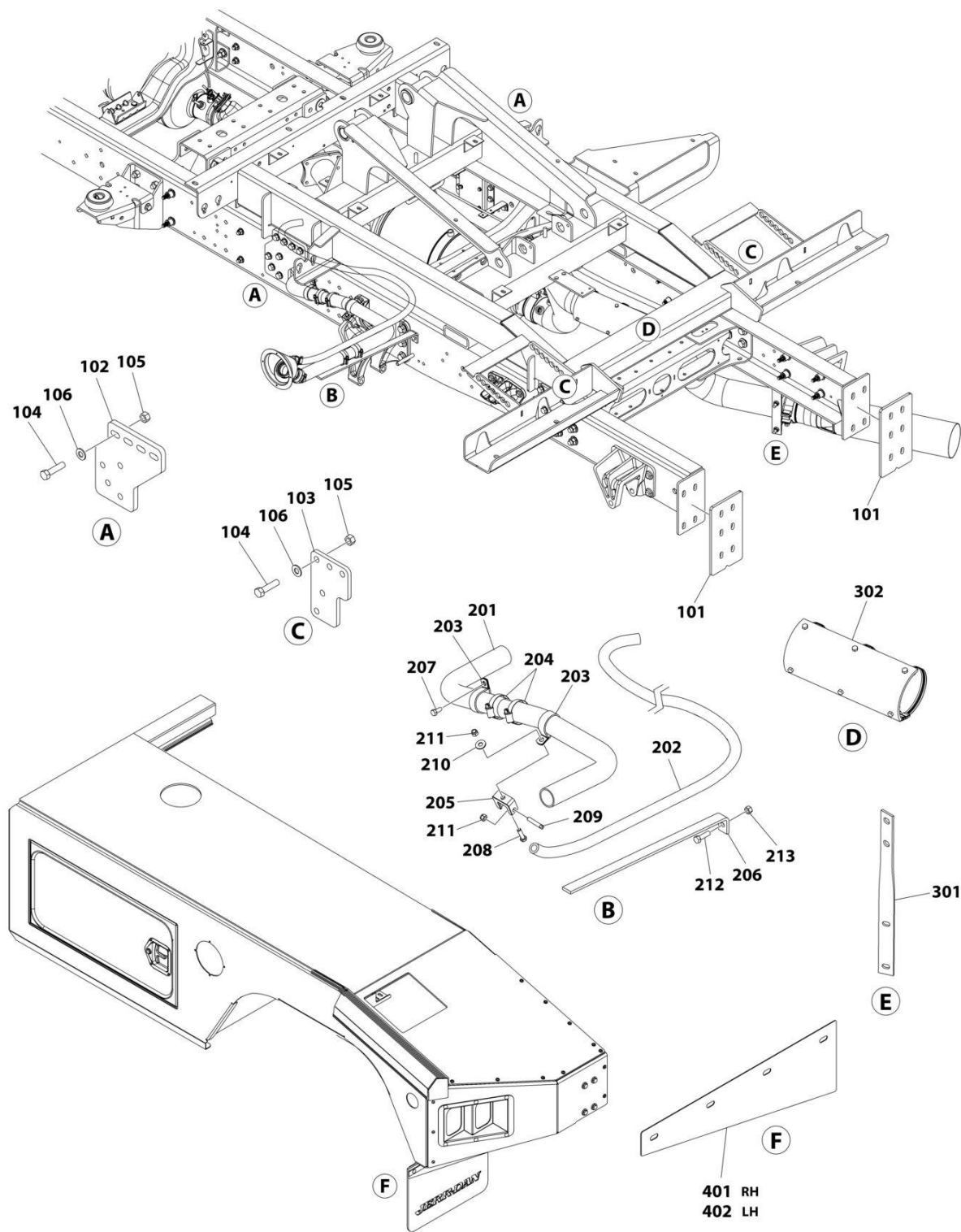
FIGURE 1-10. CHASSIS MOUNTING KIT - CV515 2019+ WITH 141IN WB
