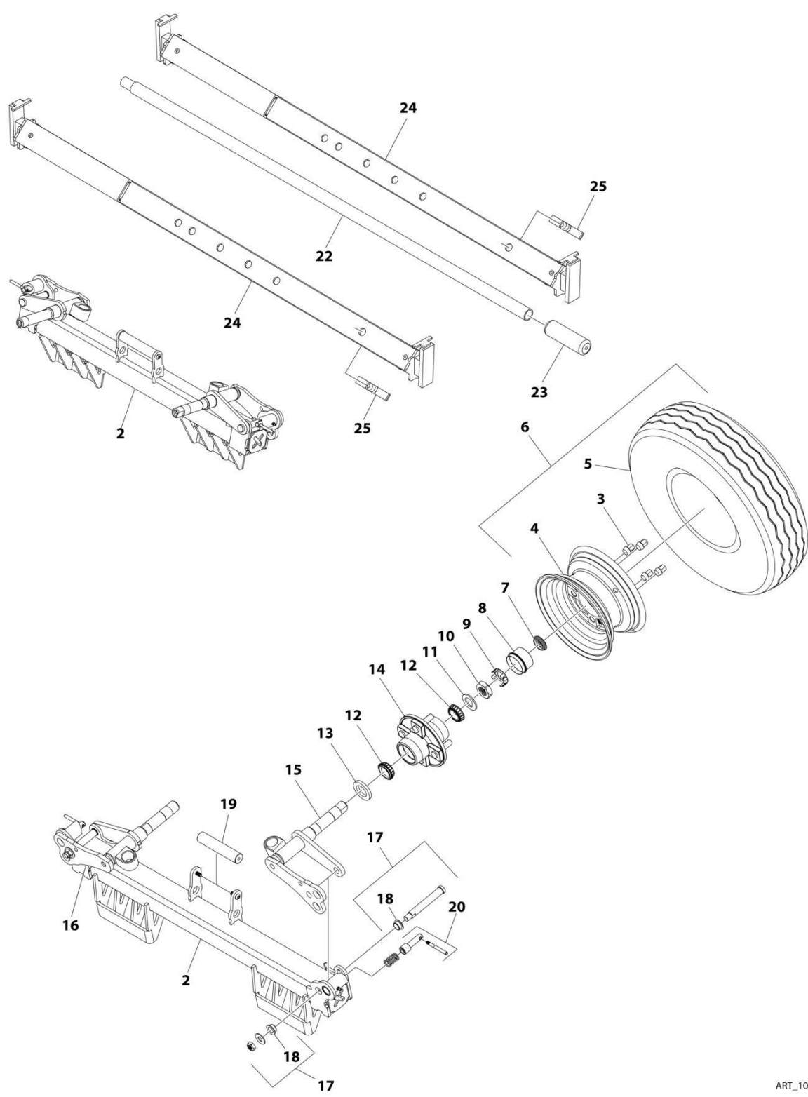
FIGURE 9-3. DOLLIES ASSEMBLY
