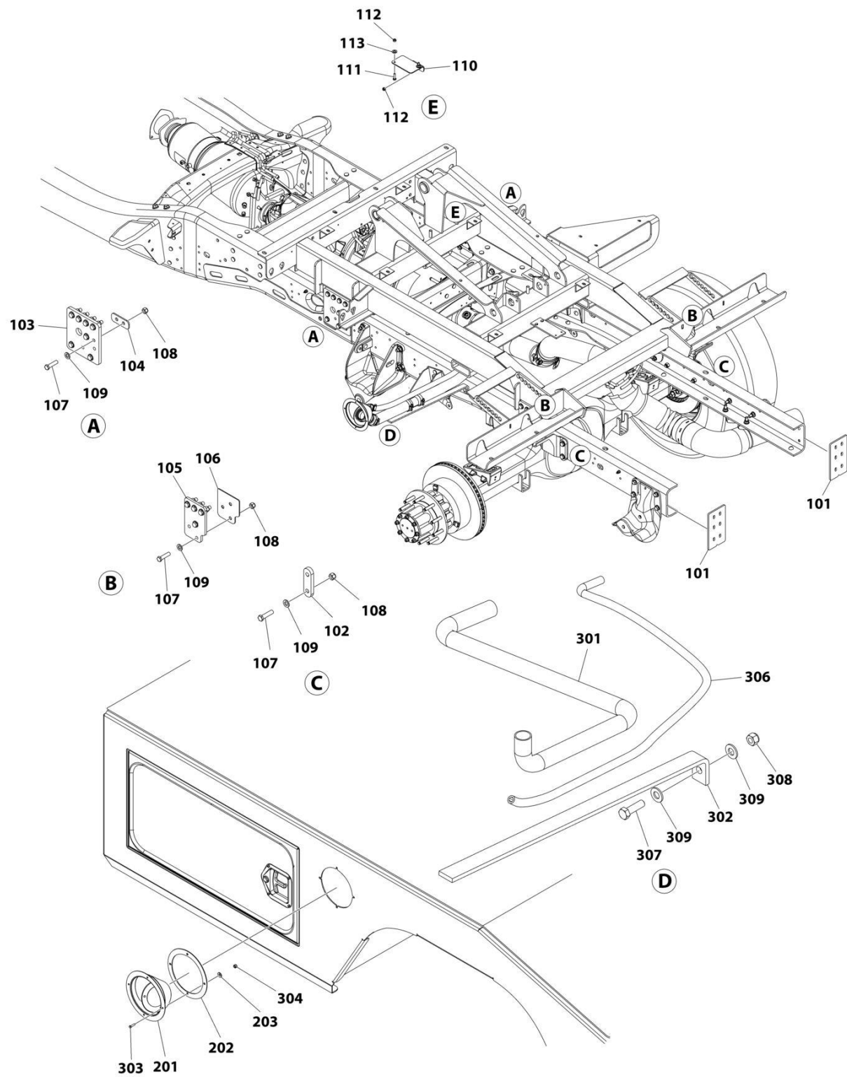
FIGURE 1-4. CHASSIS MOUNTING KIT - DODGE 2013+ WITH 84IN CA
