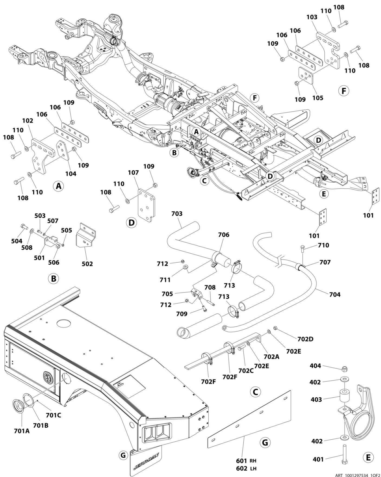
FIGURE 1-5. CHASSIS MOUNTING KIT - FORD DIESEL 2017+ WITH 60IN CA
