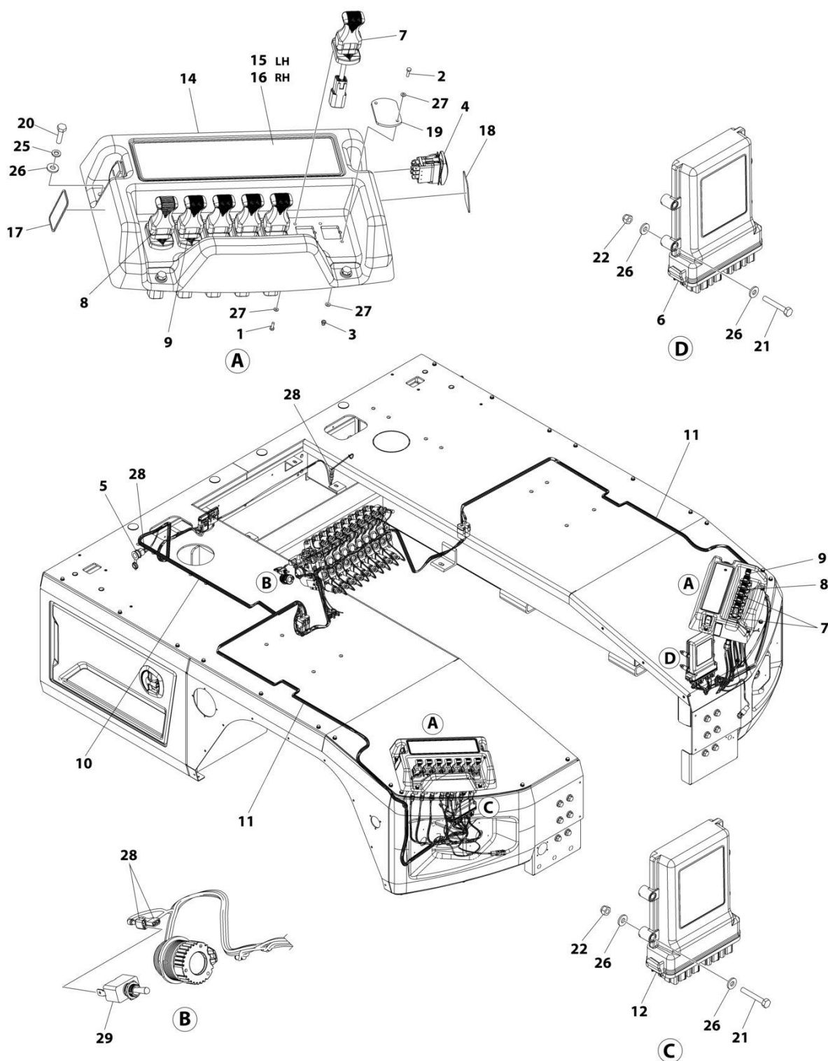
FIGURE 5-3. CONTROLS INSTALLATION - 16 FUNCTION (MANUAL GRID)
