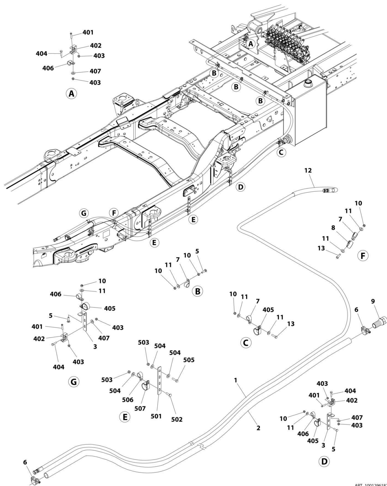
FIGURE 6-21. HOSE AND CLAMP INSTALLATION (FORD PTO - 203IN WB)
