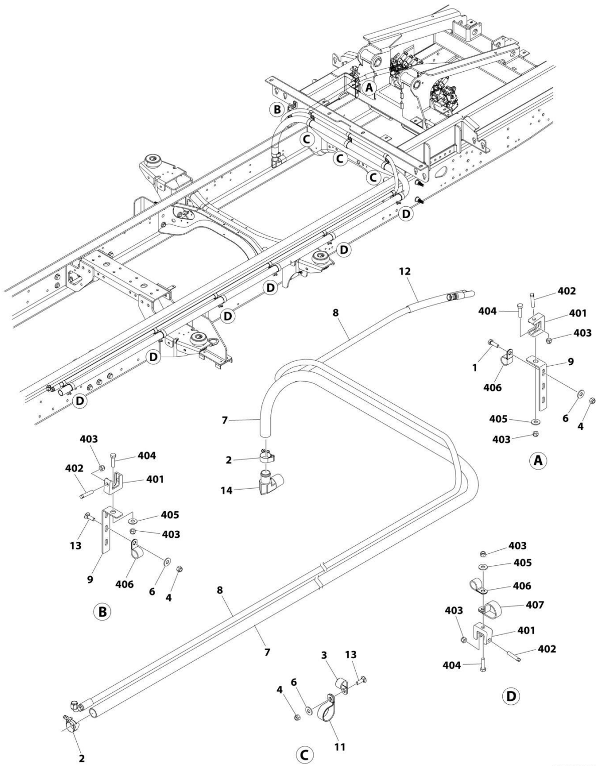
FIGURE 6-13. HOSE AND CLAMP INSTALLATION (CV515 - 199IN WB)
