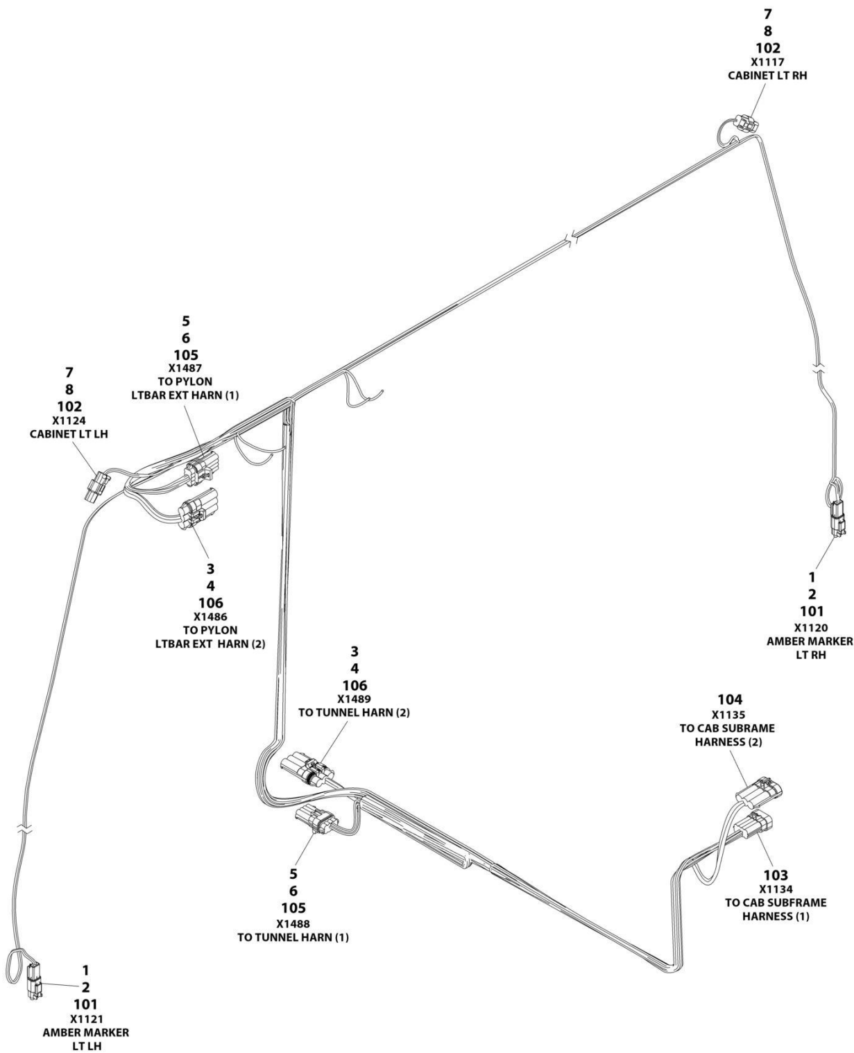
FIGURE 7-40. TUNNEL HARNESS
