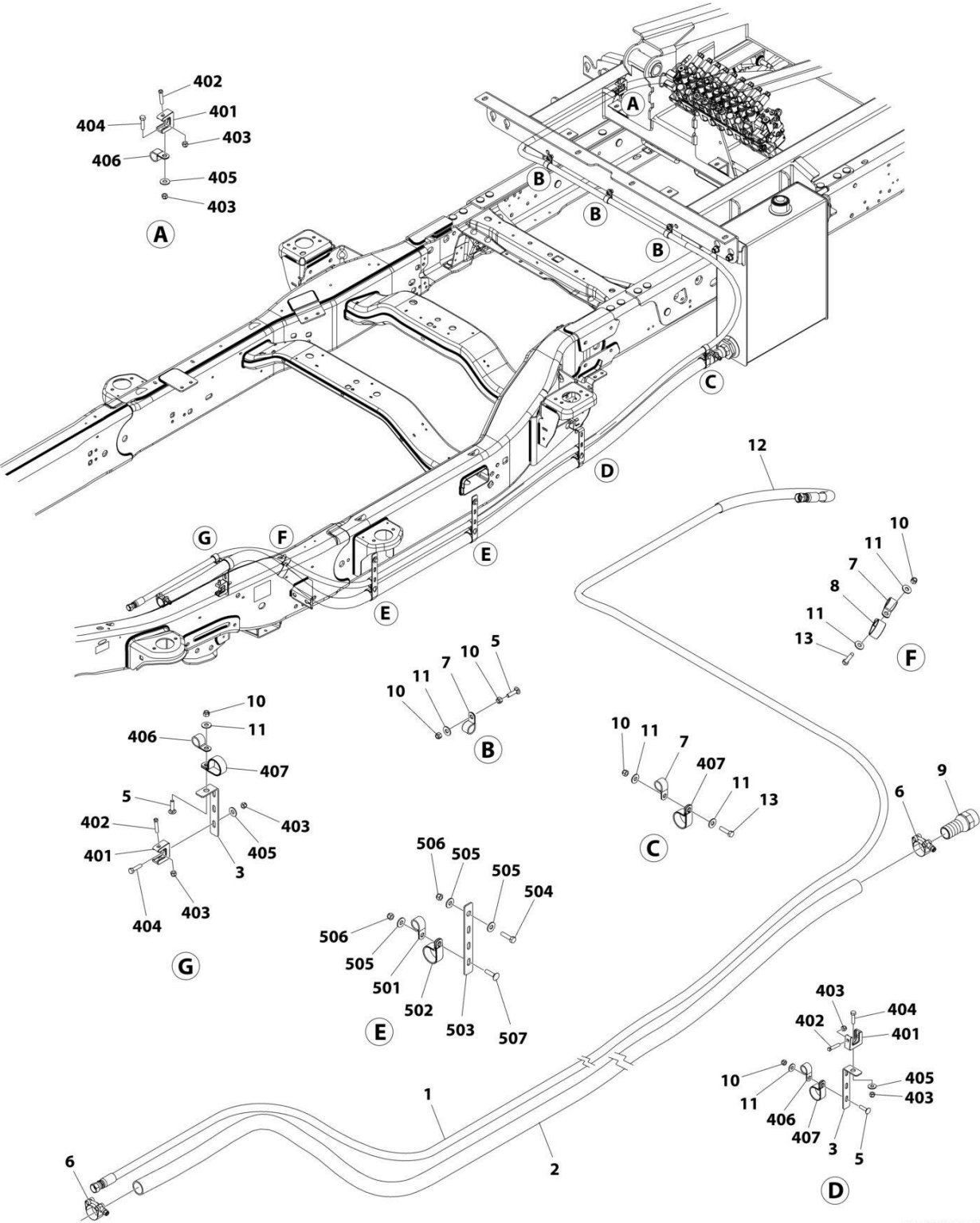
FIGURE 6-20. HOSE AND CLAMP INSTALLATION (FORD PTO - 192IN WB)
