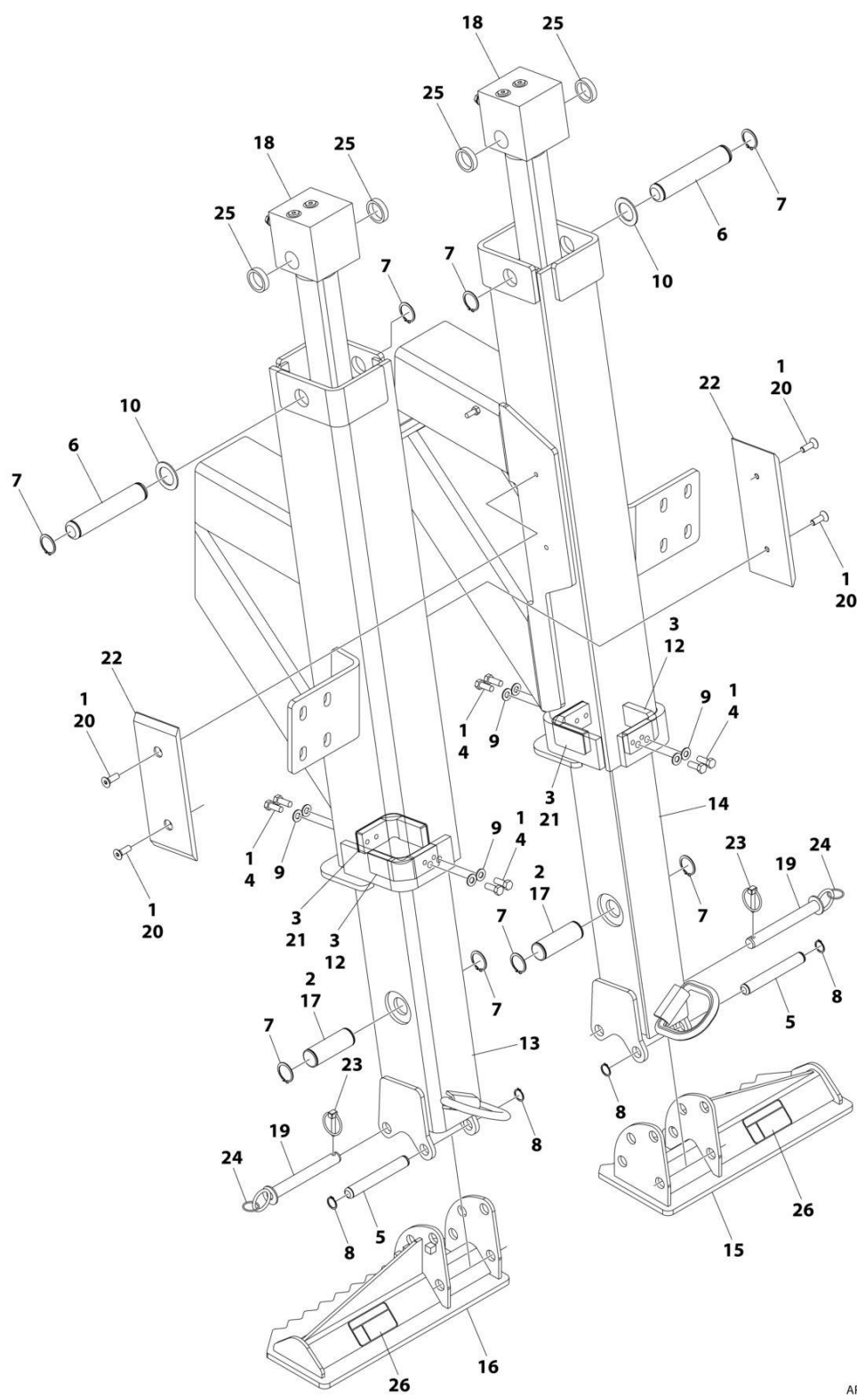
FIGURE 1-14. REAR HYDRAULIC SPADES INSTALLATION
