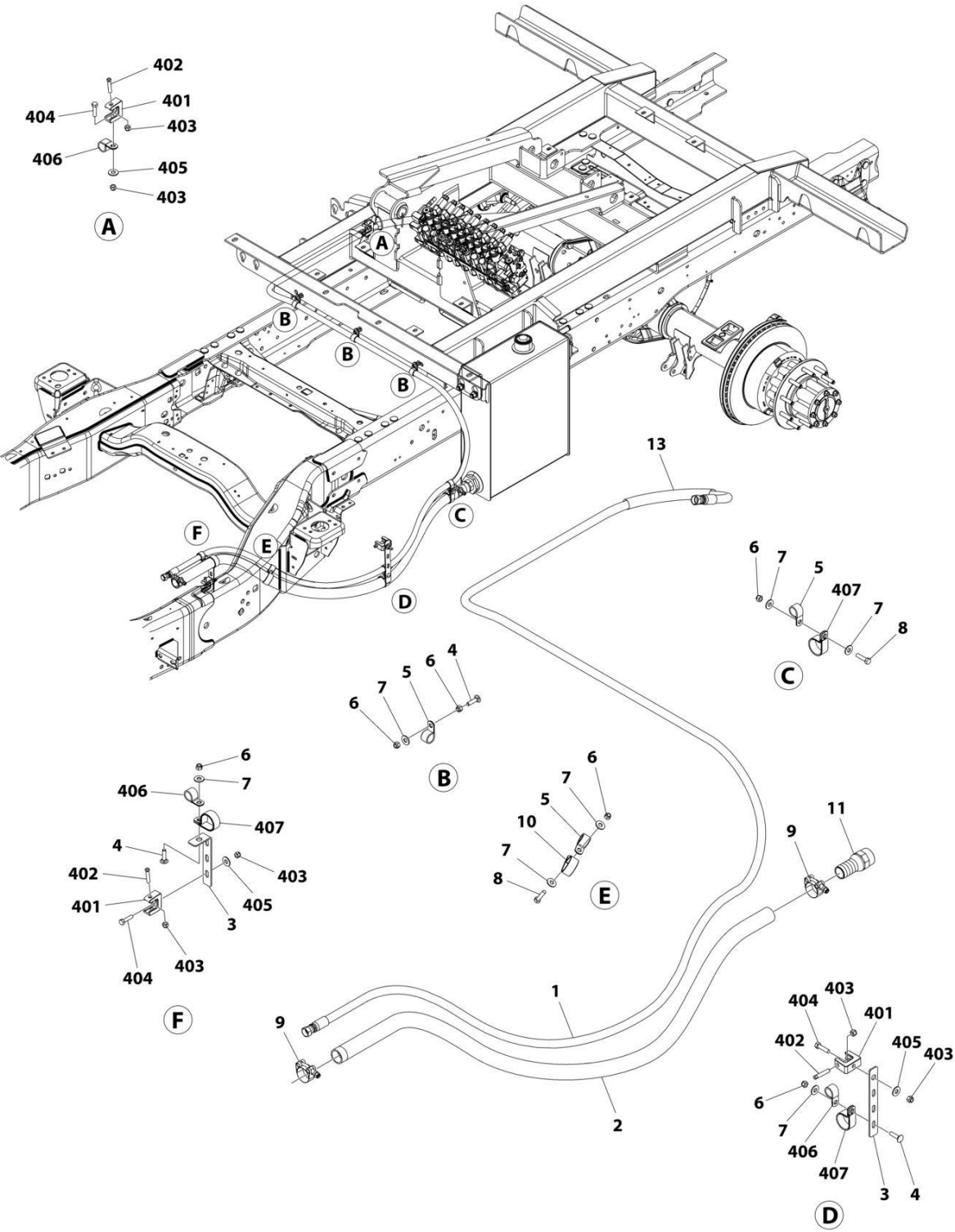
FIGURE 6-17. HOSE AND CLAMP INSTALLATION (FORD PTO - 145IN WB)
