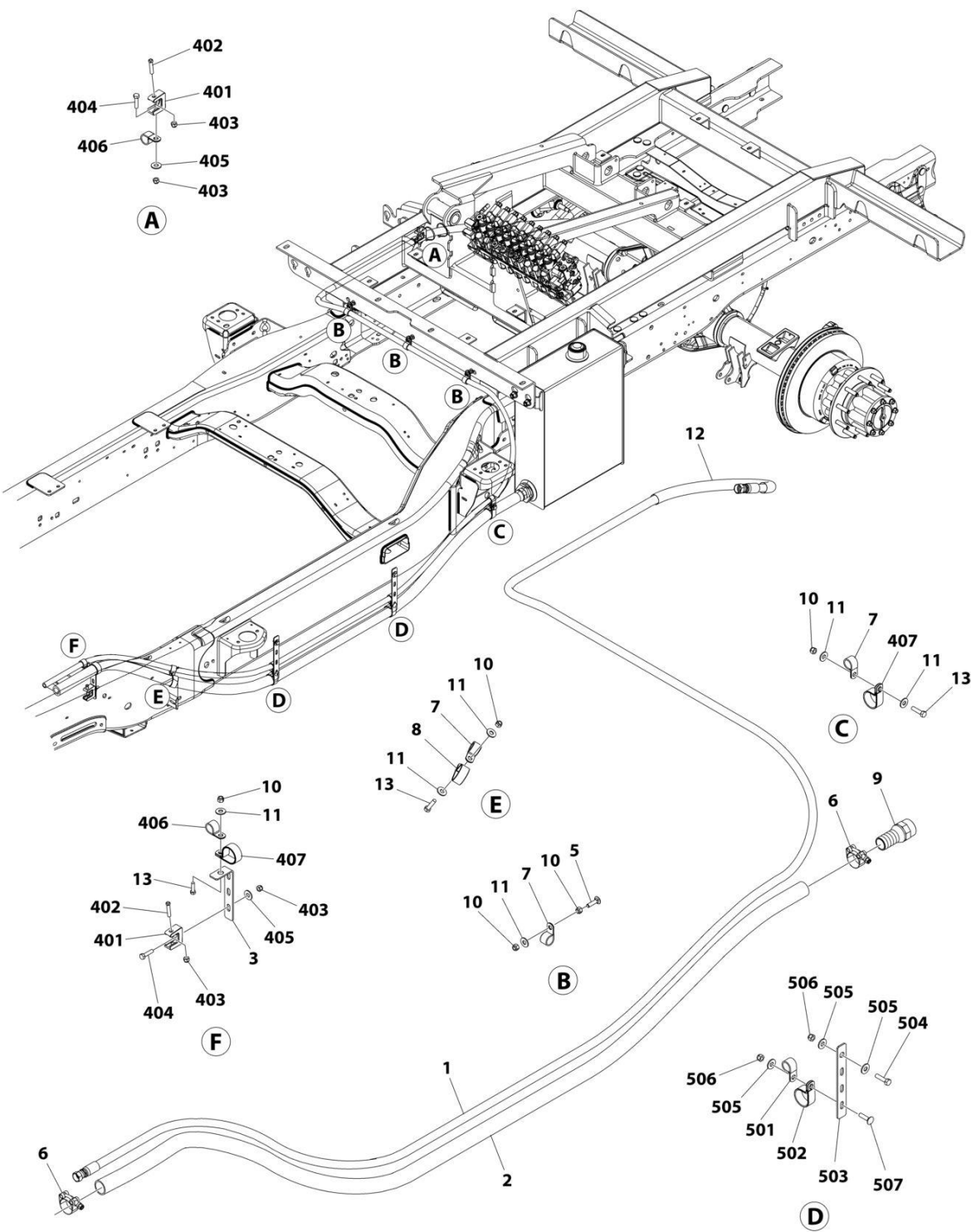
FIGURE 6-19. HOSE AND CLAMP INSTALLATION (FORD PTO - 179IN WB)
