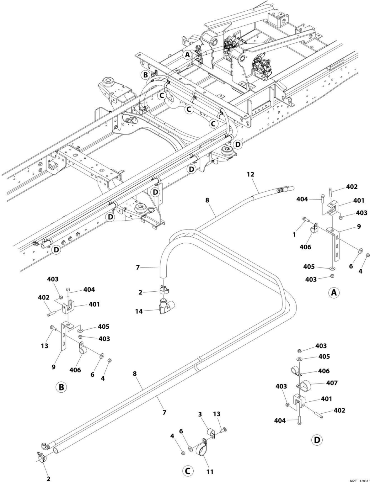
FIGURE 6-12. HOSE AND CLAMP INSTALLATION (CV515 - 175IN WB)
