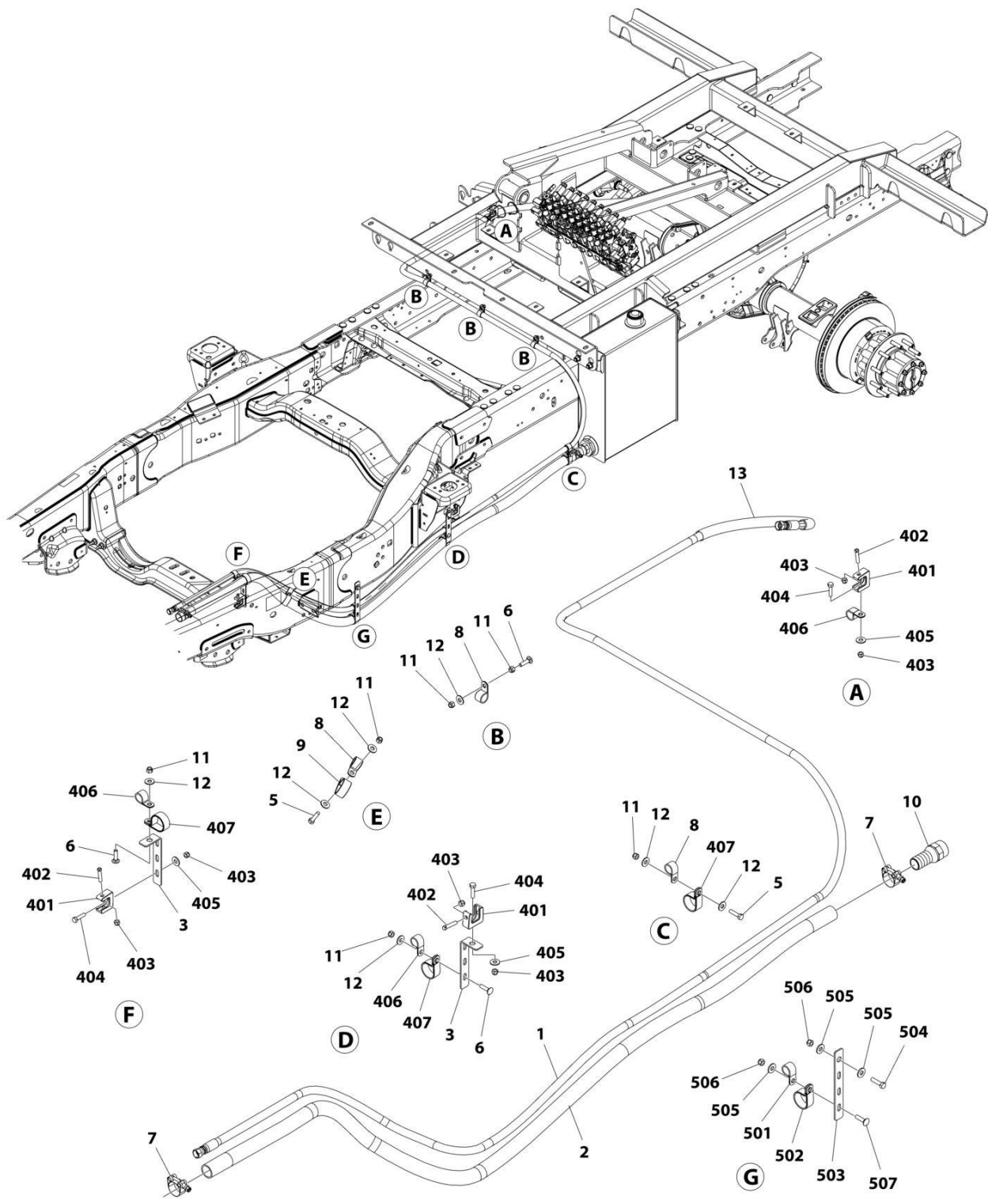
FIGURE 6-18. HOSE AND CLAMP INSTALLATION (FORD PTO - 167-169IN WB)
