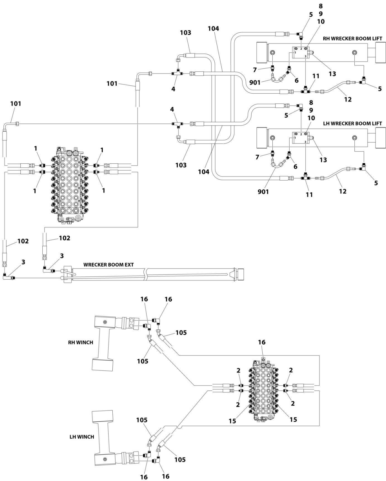
FIGURE 6-2. HOSE INSTALLATION - STANDARD
