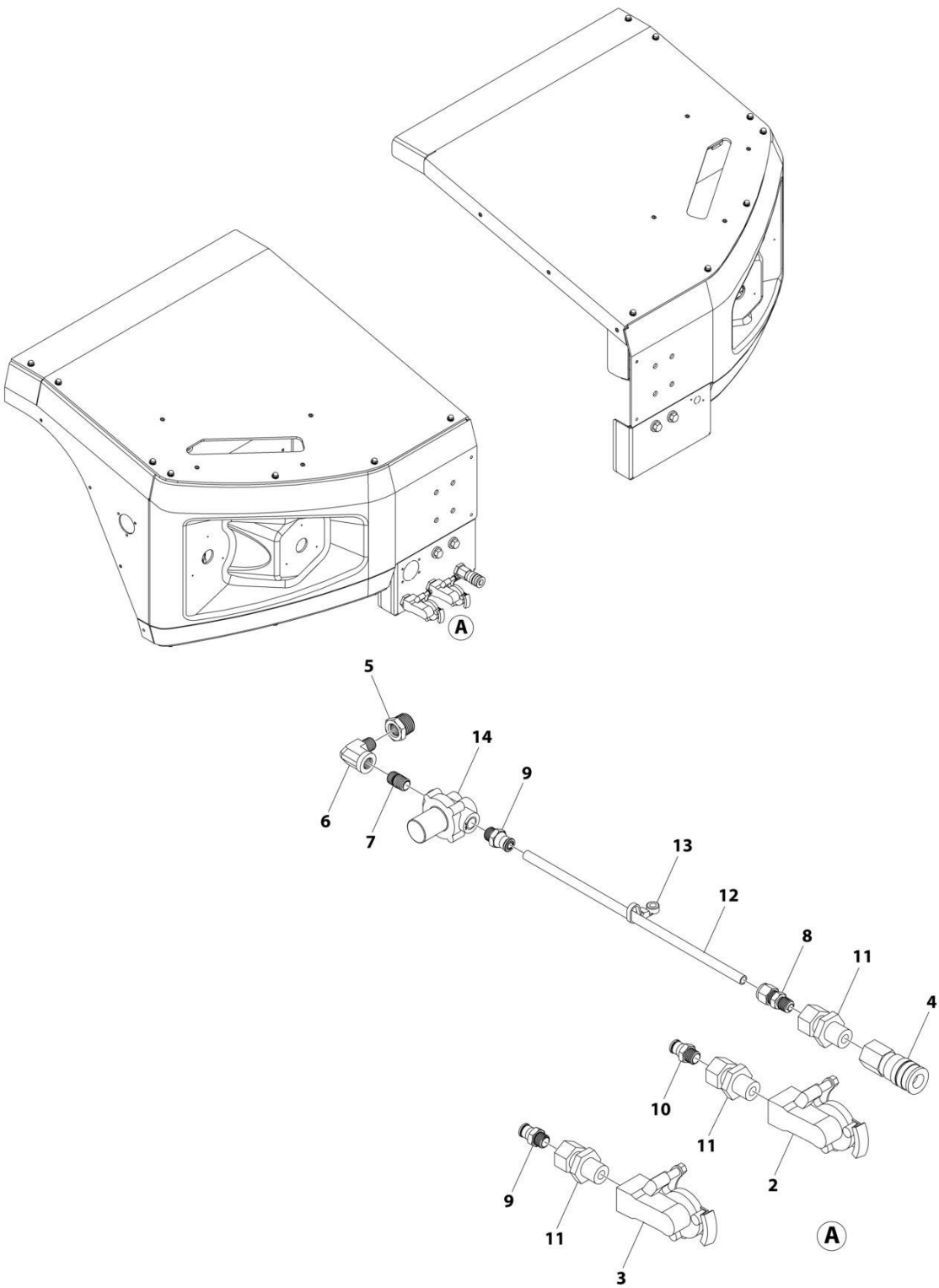
FIGURE 6-1. GLADHAND & AUX AIR INSTALLATION
