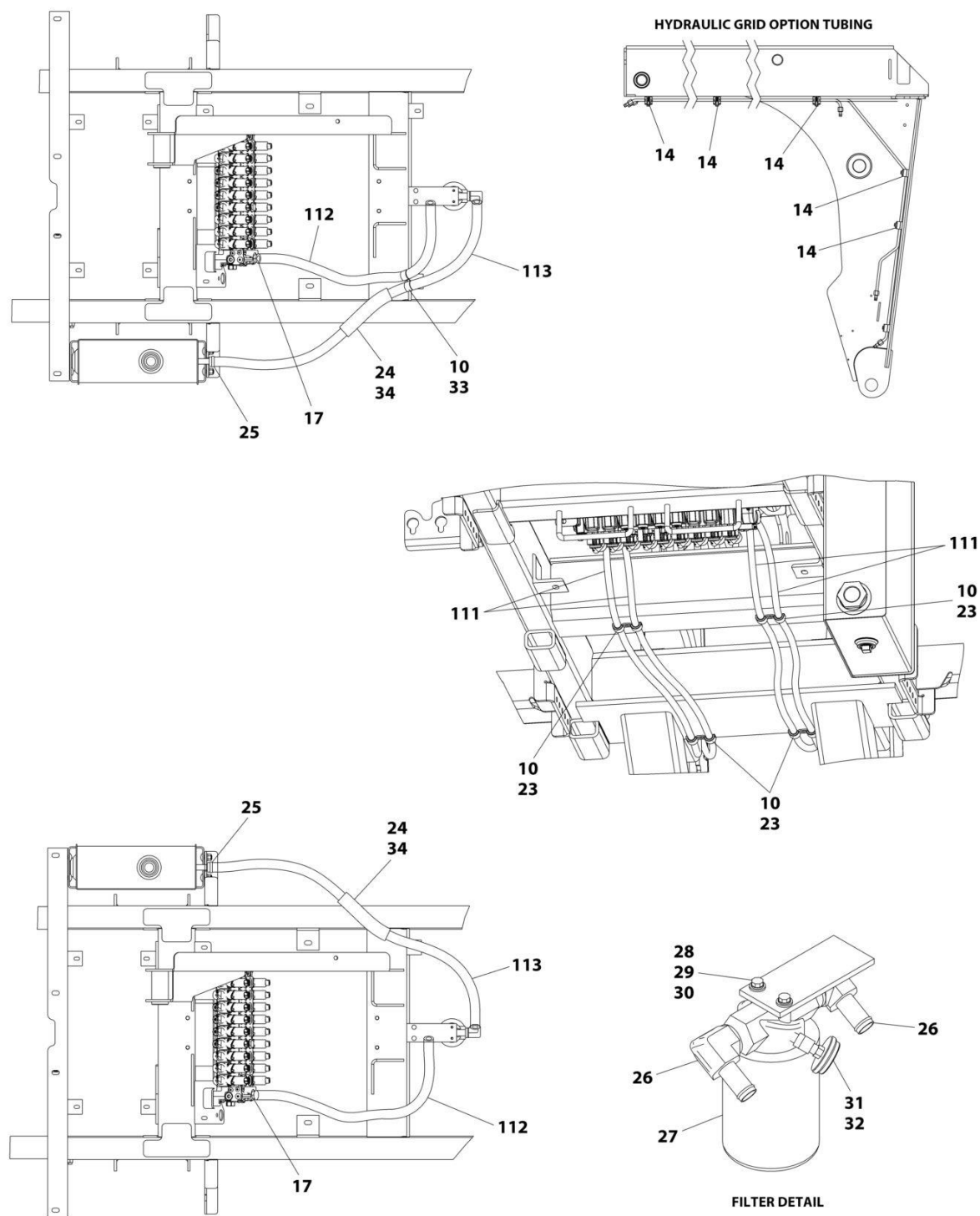
FIGURE 6-4. HOSE INSTALLATION - STANDARD
