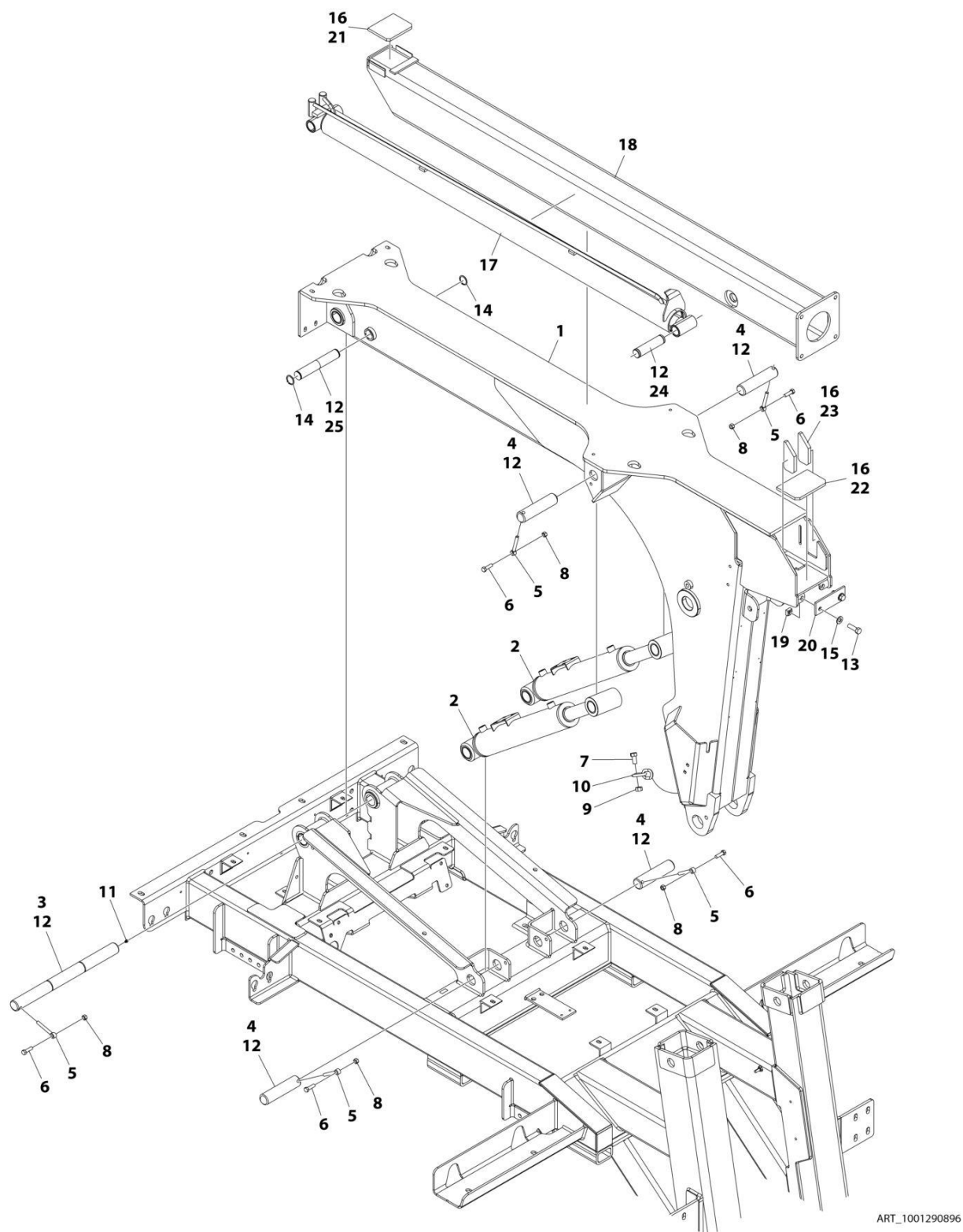
FIGURE 2-1. MAIN BOOM INSTALLATION (WITH FLY BOOM)
