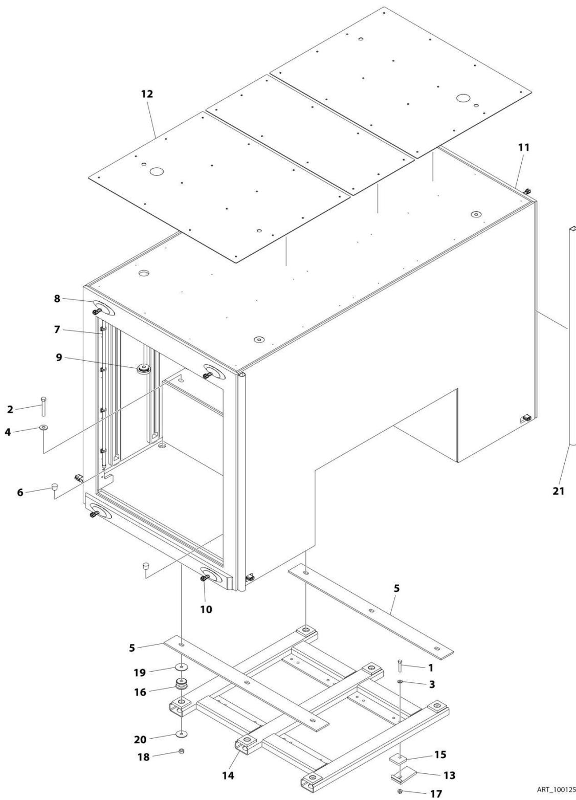
FIGURE 4-87. TUNNEL INSTALLATION (49IN WITHOUT BATTERY) (B SLOT)
