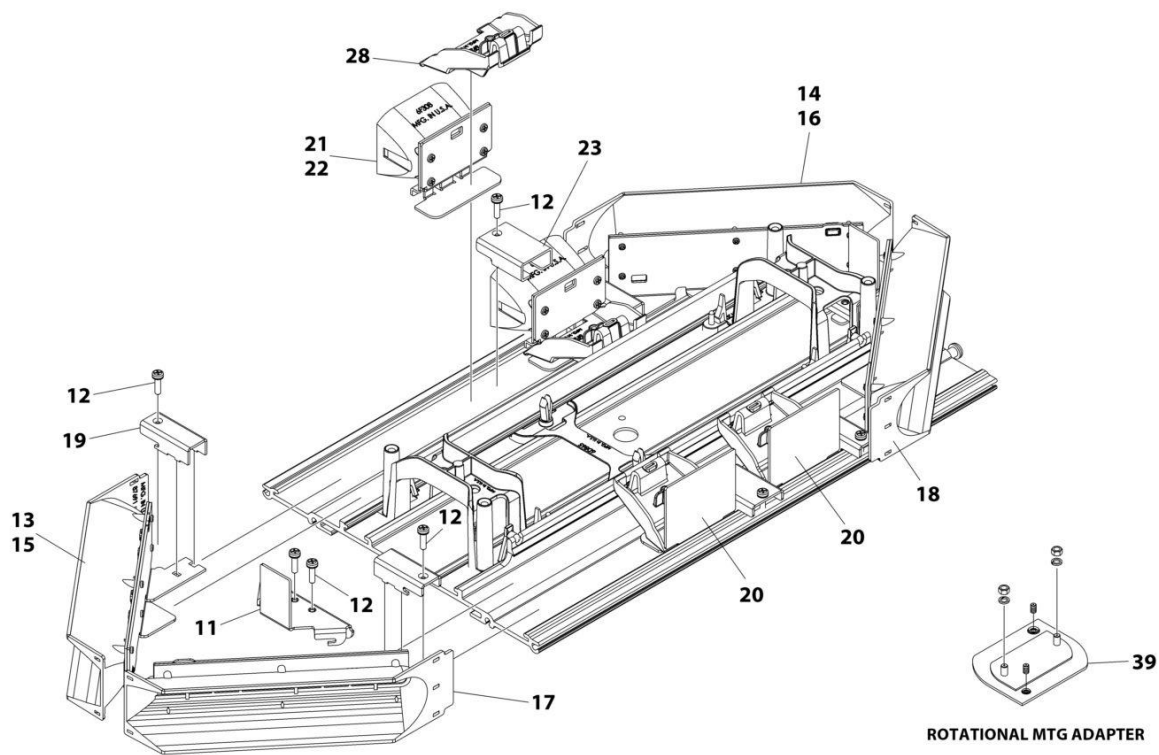
FIGURE 7-47. LIGHTS - LAMP ASSEMBLY - 22IN WHELEN WING LIGHT
