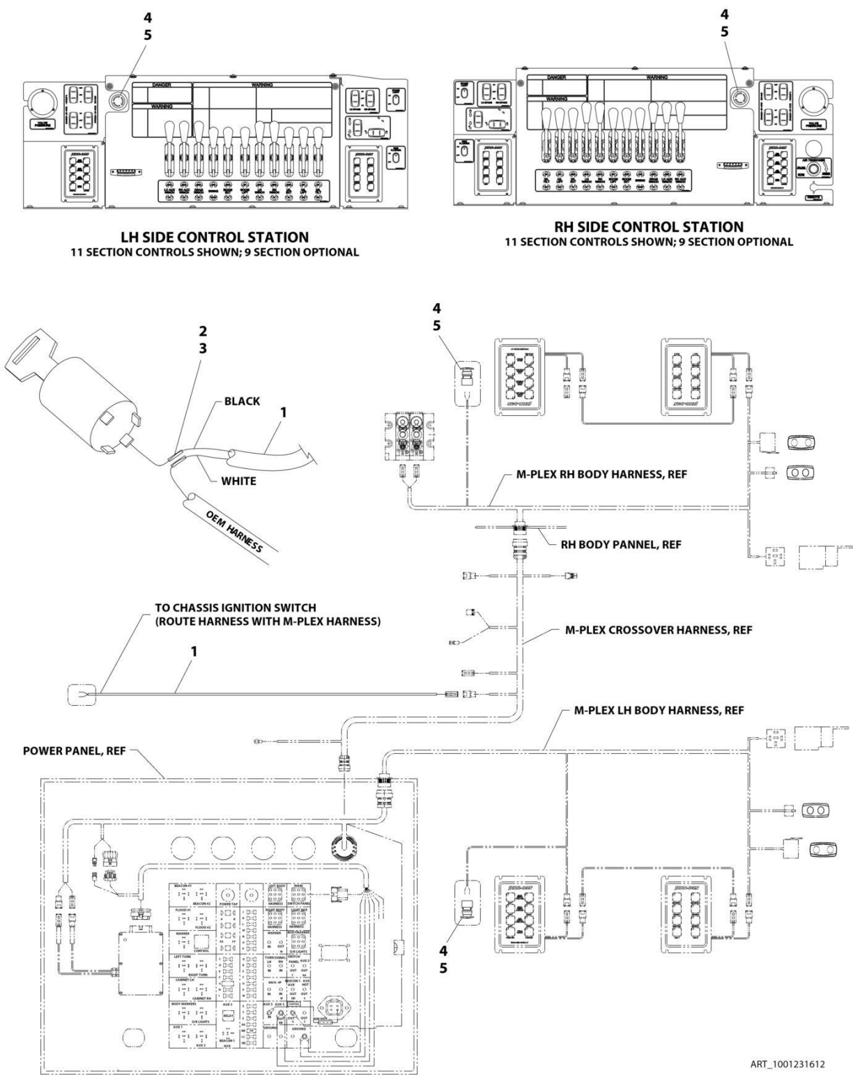
FIGURE 5-11. EMERGENCY STOP INSTALLATION
