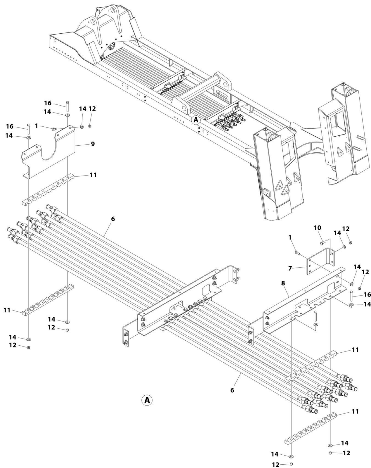
FIGURE 6-21. TUBE INSTALLATION - SUBFRANE (SN 0230007638 through 0230011033, Excluding 0230010775, 0230010821 and 0230010823)
