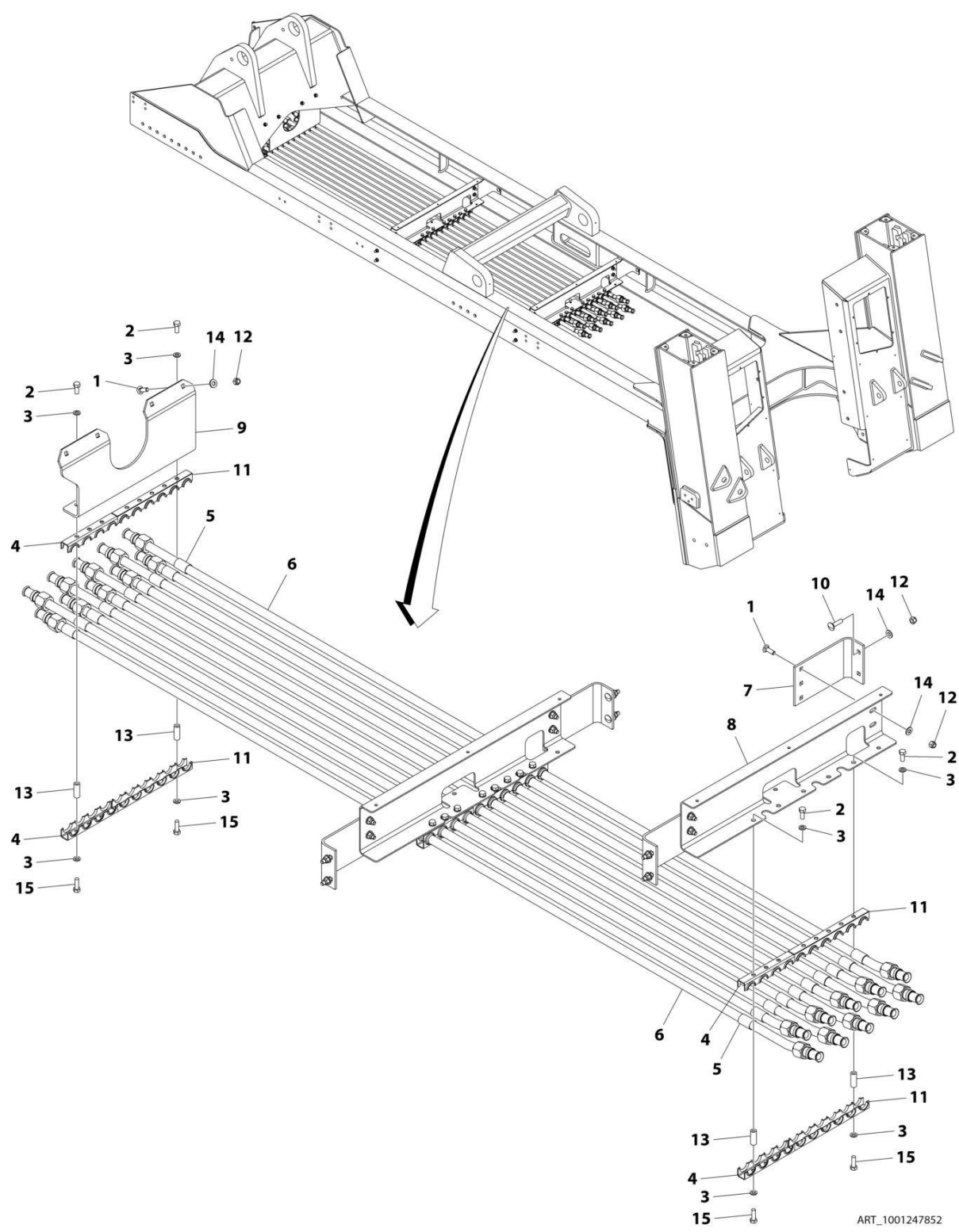
FIGURE 6-20. TUBE INSTALLATION - SUBFRANE (Prior to SN 0230007637)
