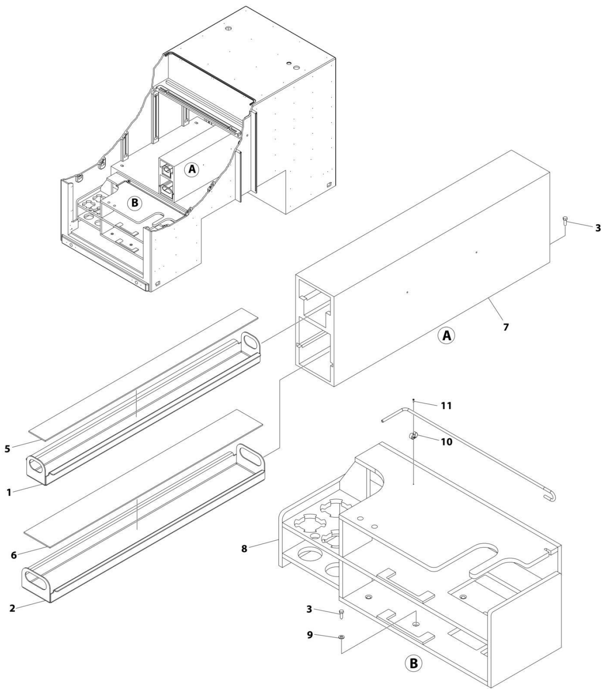
FIGURE 9-32. TIRE LIFT STORAGE INSTALLATION, 48IN
