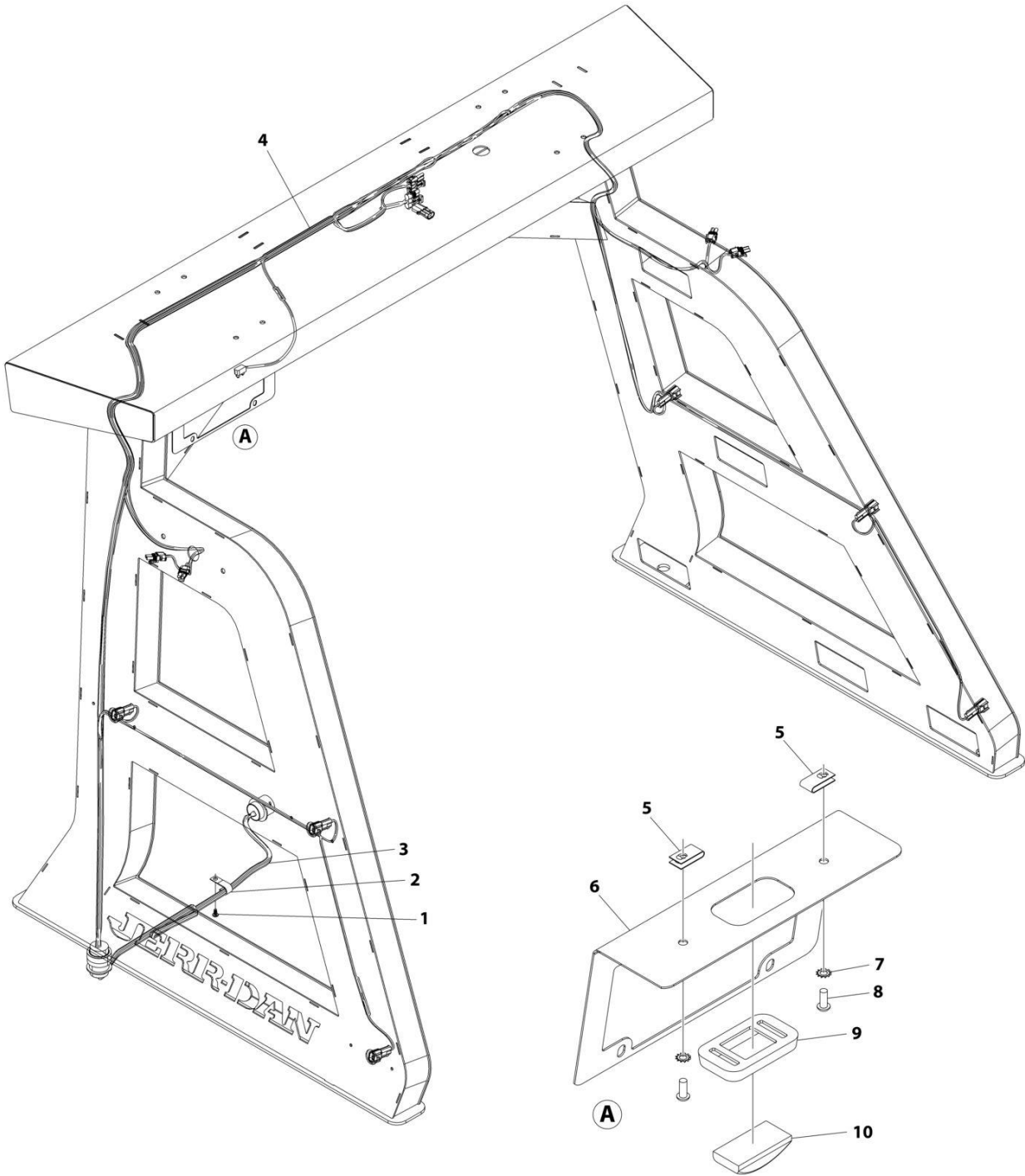
FIGURE 7-51. PYLON ELECTRICAL INSTALLATION (57IN PYLON)
