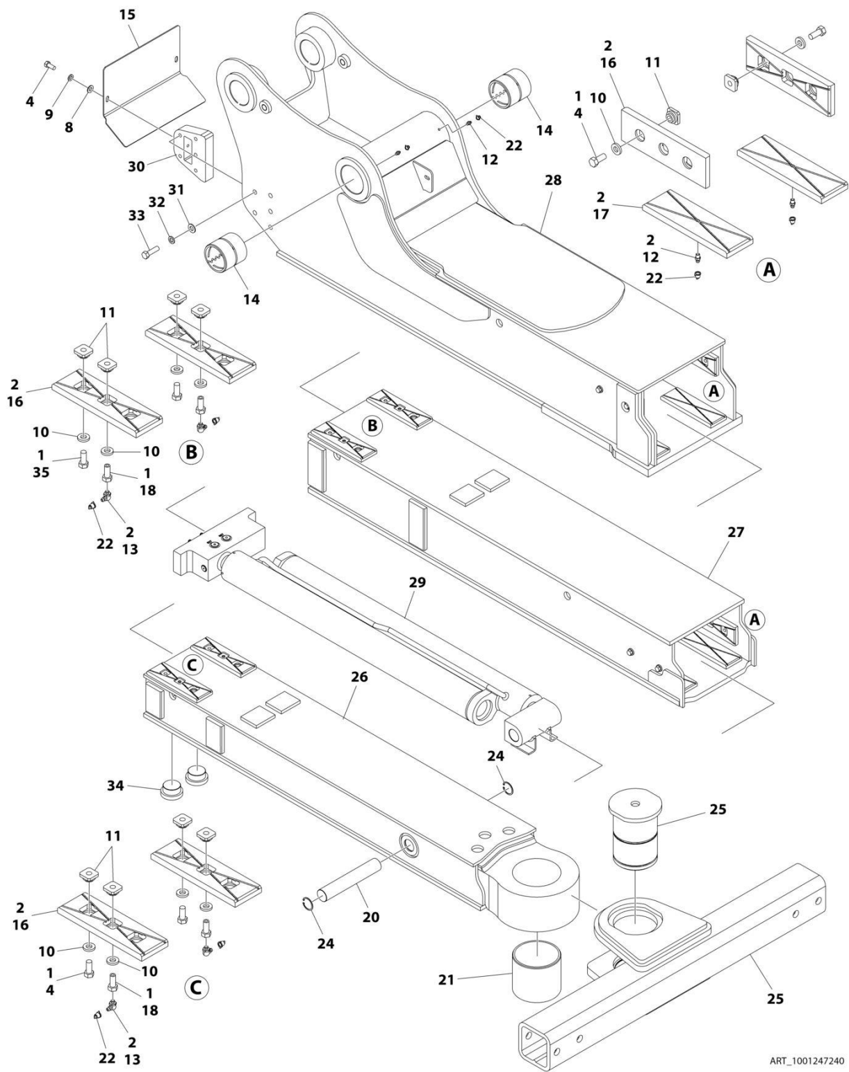
FIGURE 3-2. UNDERLIFT ASSEMBLY
