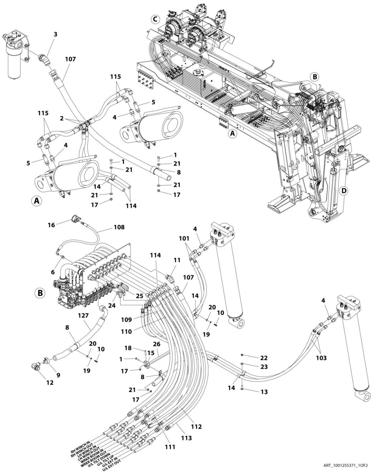
FIGURE 6-8. HYDRAULIC INSTALLATION - BASE 25T INT
