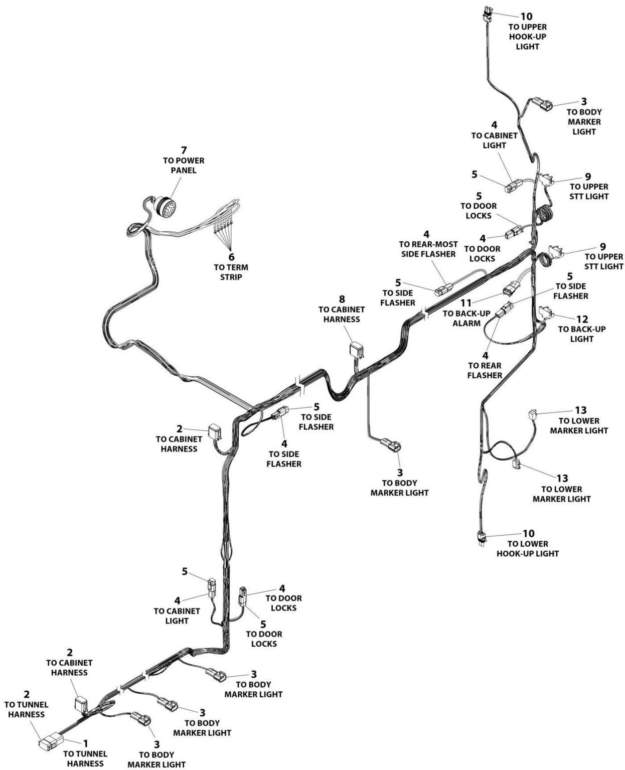
FIGURE 7-7. BODY HARNESS (LH)
