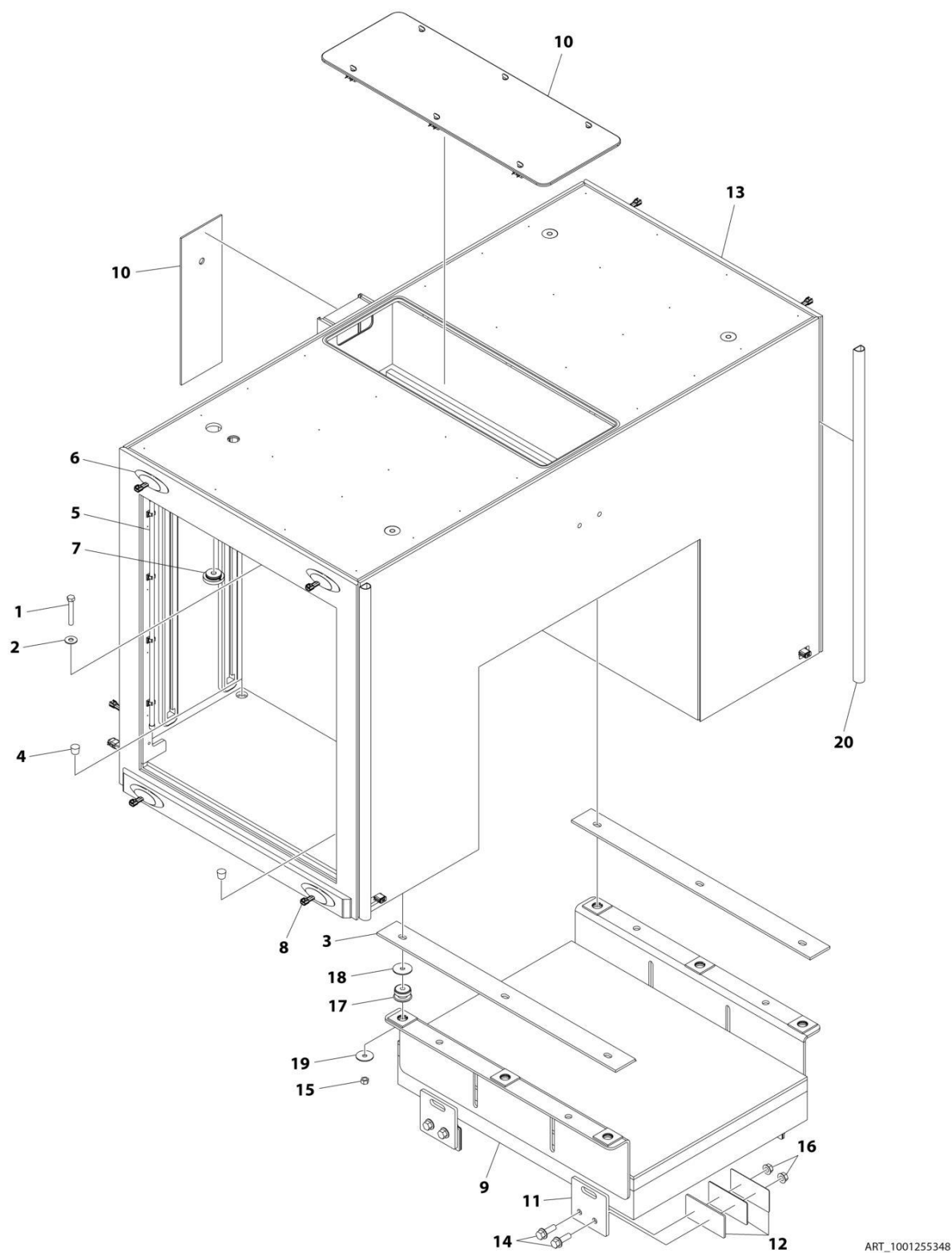
FIGURE 4-89. TUNNEL INSTALLATION (51IN TUNNEL WITH 4500 LBS COUNTERWEIGHT)
