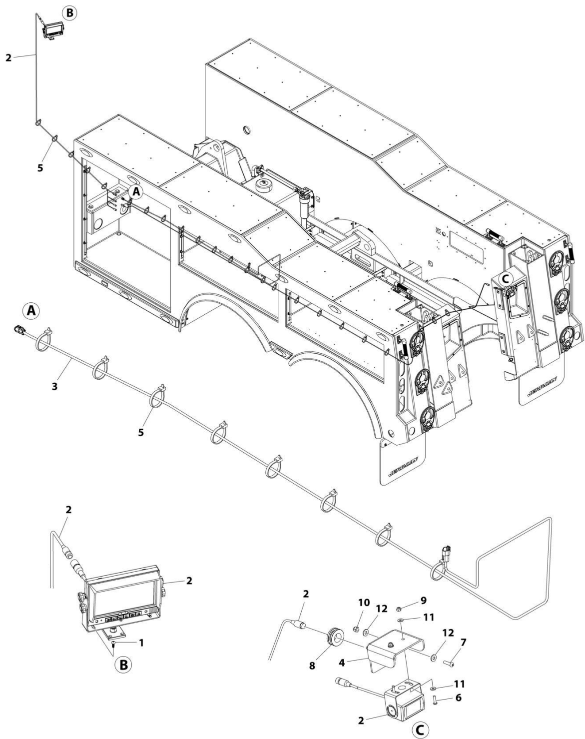
FIGURE 9-5. CAMERA INSTALLATION - BACK-UP (SN 0230009519 through 0230011033, Excluding 0230010775, 0230010821 and 0230010823)
