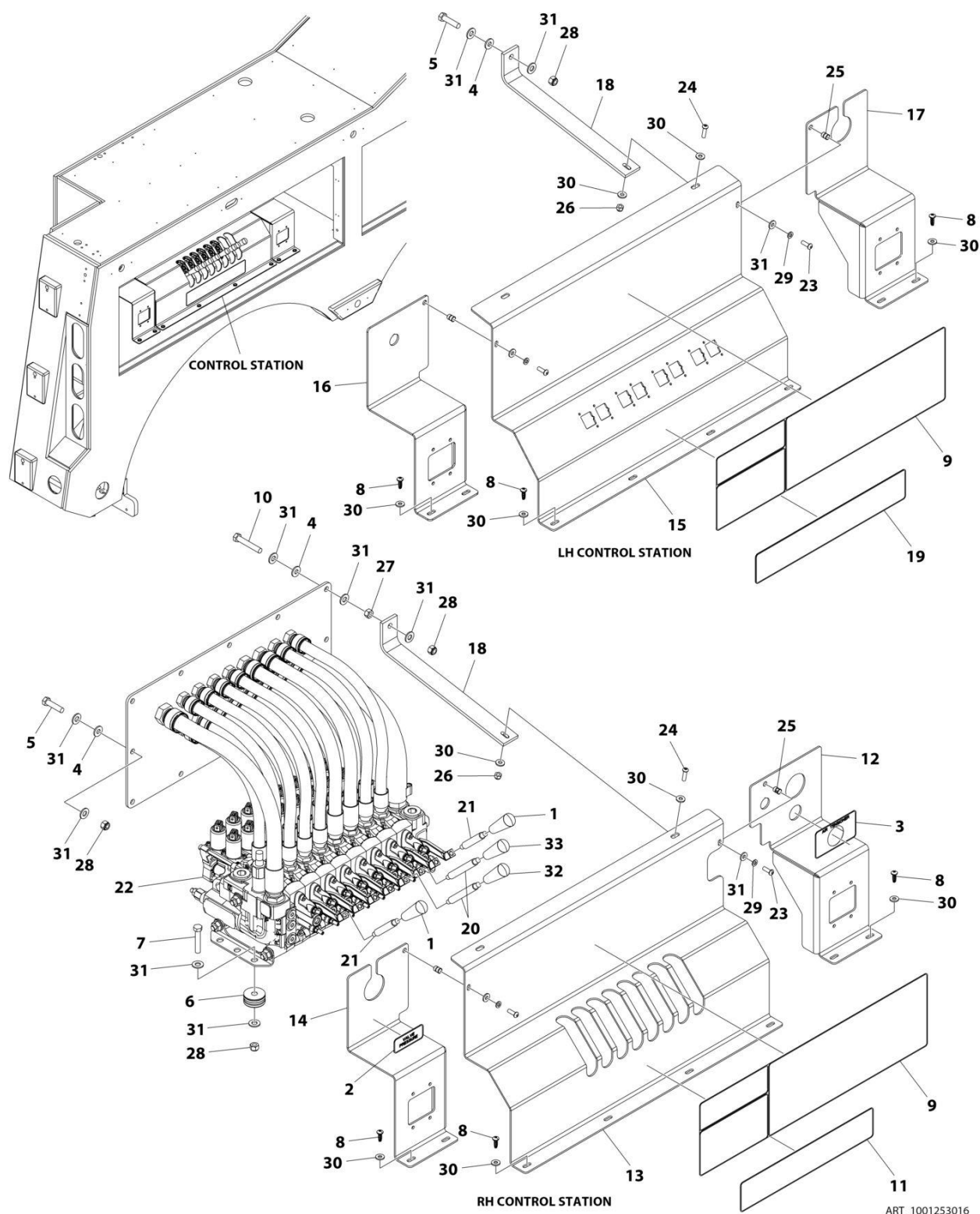
FIGURE 5-1. CONTROLS VALVE INSTALLATION, 8 SECTION - 8 SOLENOID (Prior to SN 0230007637)
