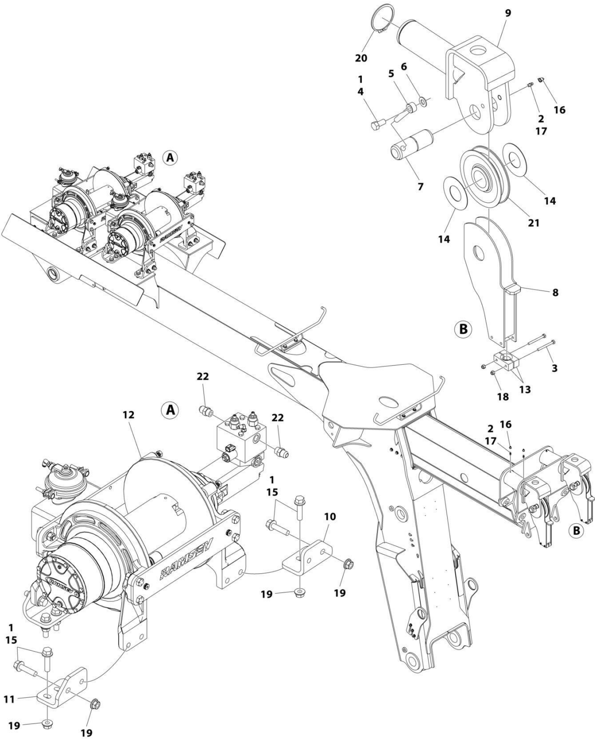
FIGURE 2-7. BOOM WINCH INSTALLATION - RAMSEY
