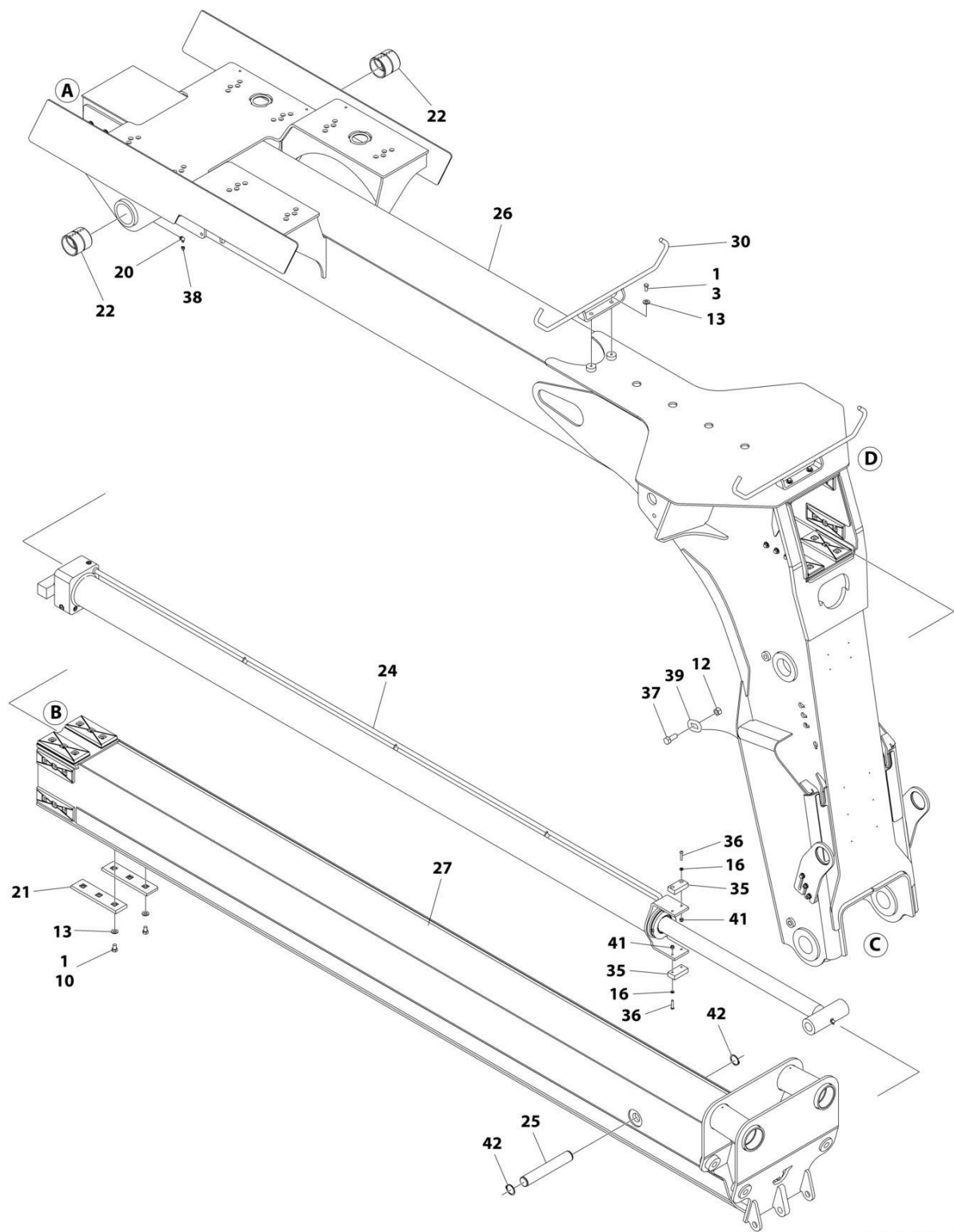
FIGURE 2-3. MAIN BOOM ASSEMBLY
