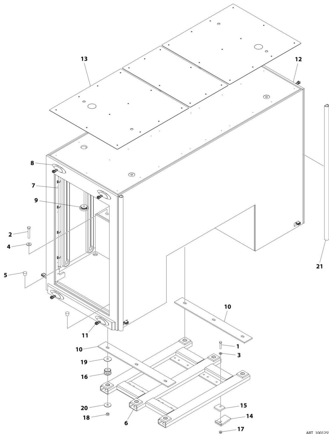
FIGURE 4-85. TUNNEL INSTALLATION (37IN WITHOUT BATTERY) (B SLOT)
