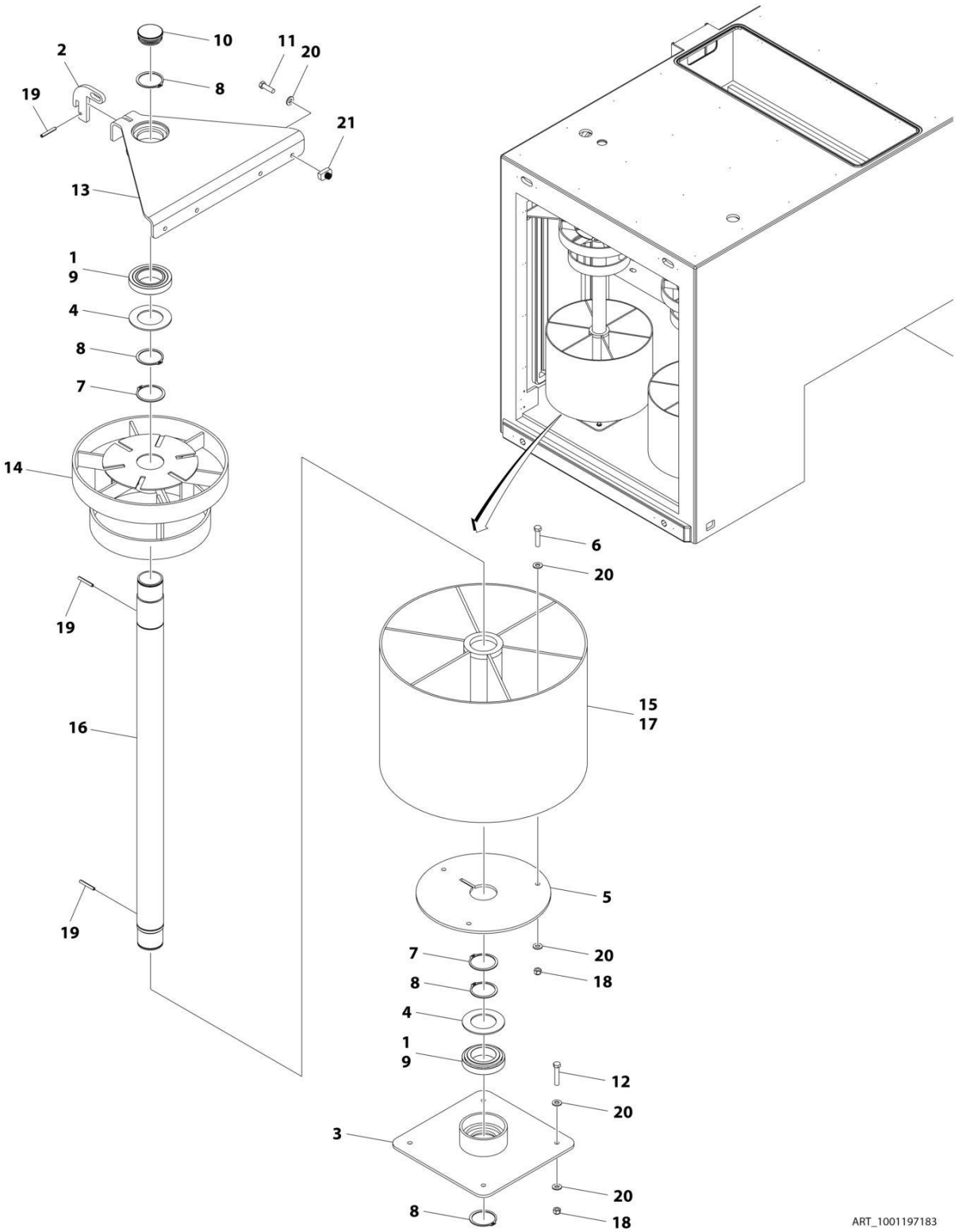
FIGURE 4-47. ROTARY TOOL RACK INSTALLATION
