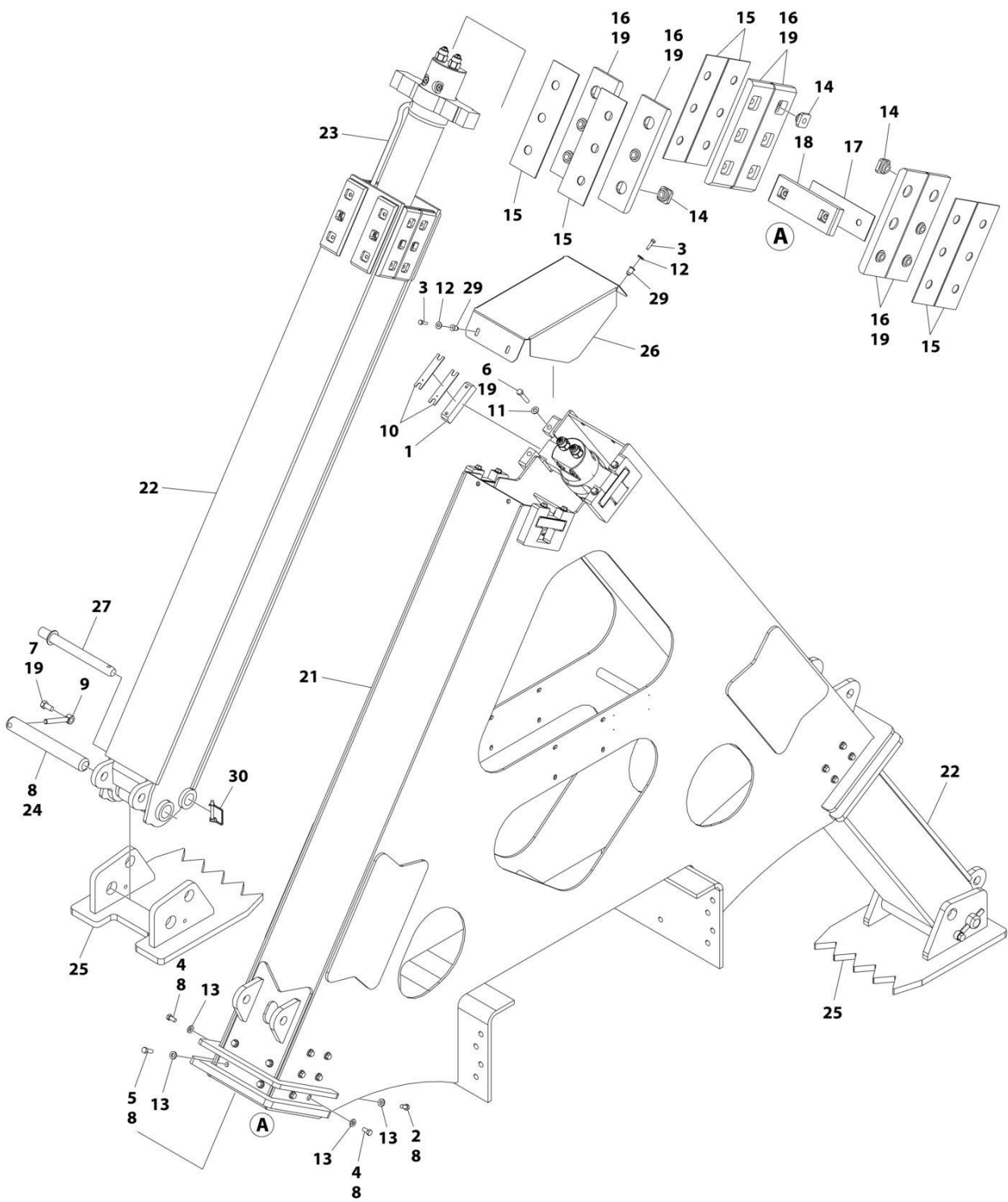
FIGURE 1-18. SIDE RECOVERY STABILIZER (SRS SS-70) ASSEMBLY
