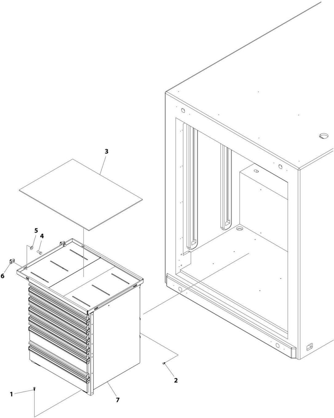
FIGURE 9-33. TOOL DRAWER INSTALLATION, TRI-AXLE
