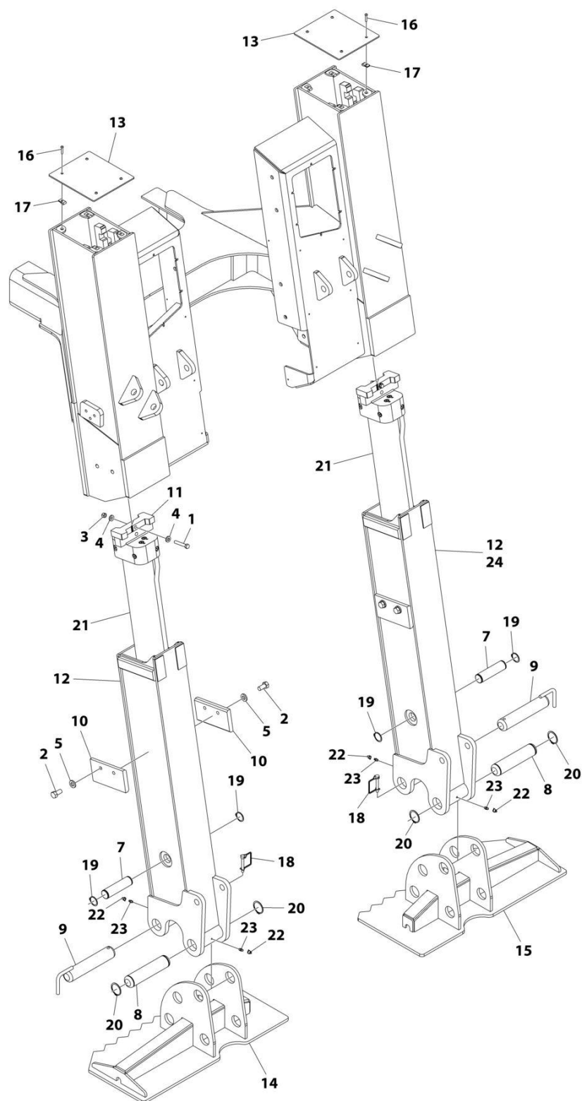
FIGURE 1-6. REAR STABILIZERS INSTALLATION (SN 0230007638 through 0230011033, Excluding 0230010775, 0230010821 and 0230010823)
