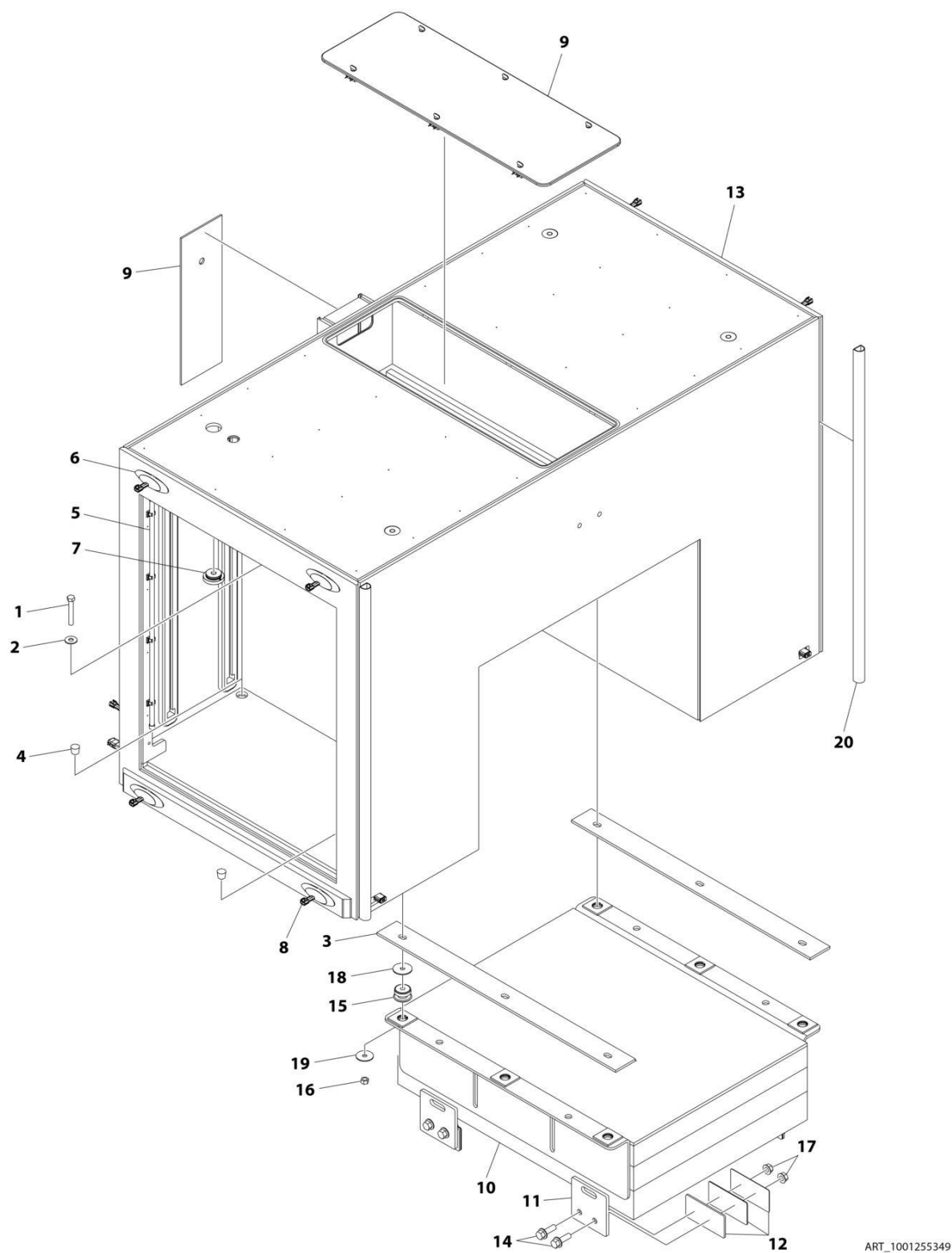
FIGURE 4-90. TUNNEL INSTALLATION (51IN TUNNEL WITH 6500 LBS COUNTERWEIGHT)
