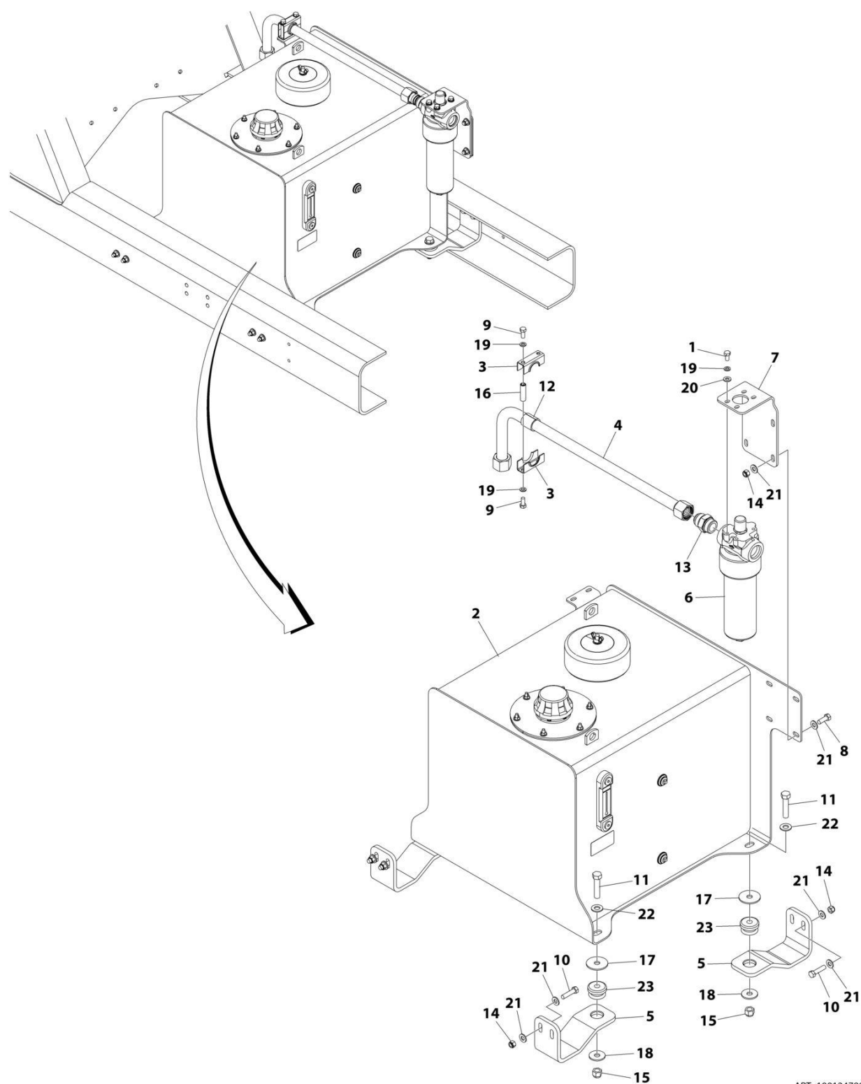
FIGURE 6-18. TANK (HYDRAULIC) INSTALLATION
