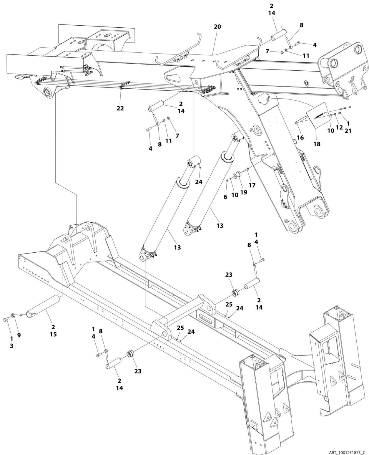
FIGURE 2-2. MAIN BOOM INSTALLATION (SN 0230007638 through 0230011033, Excluding 0230010775, 0230010821 and 0230010823)
