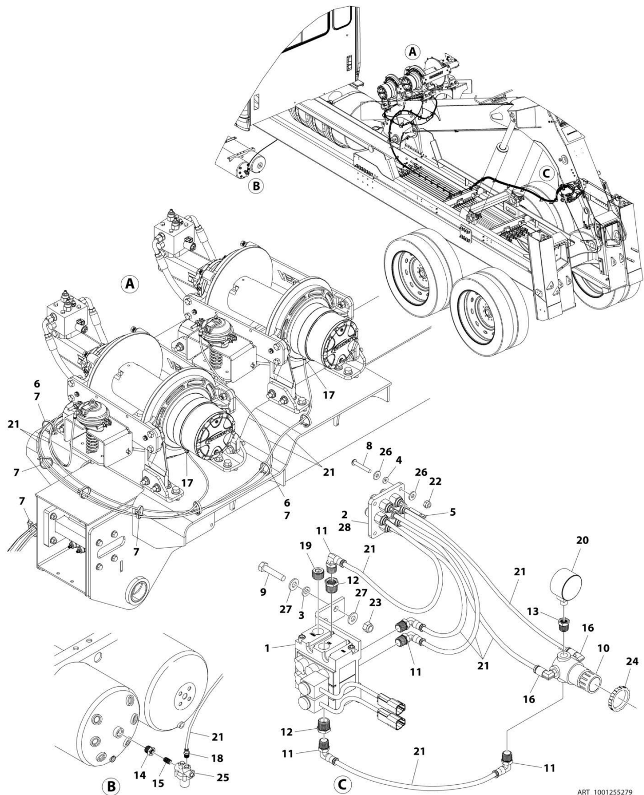
FIGURE 2-10. DUAL WINCH AIR INSTALLATION
