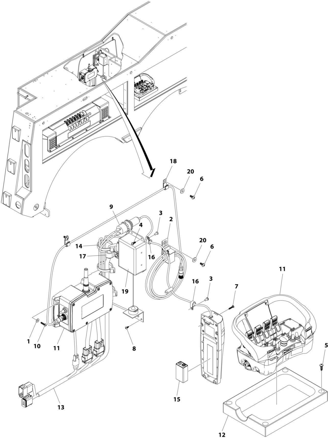
FIGURE 5-7. REMOTE CONTROLS INSTALLATION - 12 FUNCTION (CONSOLE)
