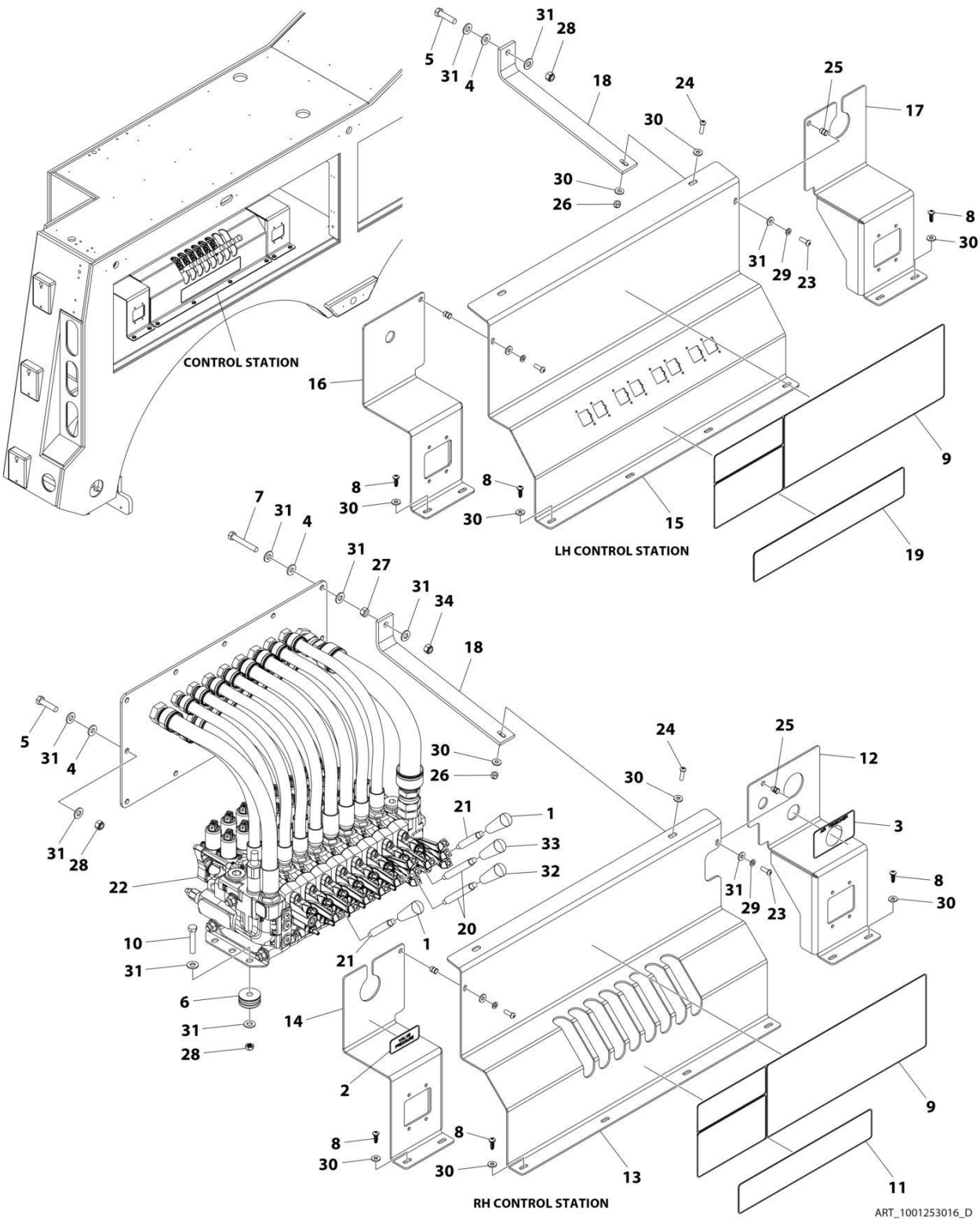
FIGURE 5-2. CONTROLS VALVE INSTALLATION, 8 SECTION - 8 SOLENOID (SN 0230007638 through 0230011033, Excluding 0230010775, 0230010821 and 0230010823)
