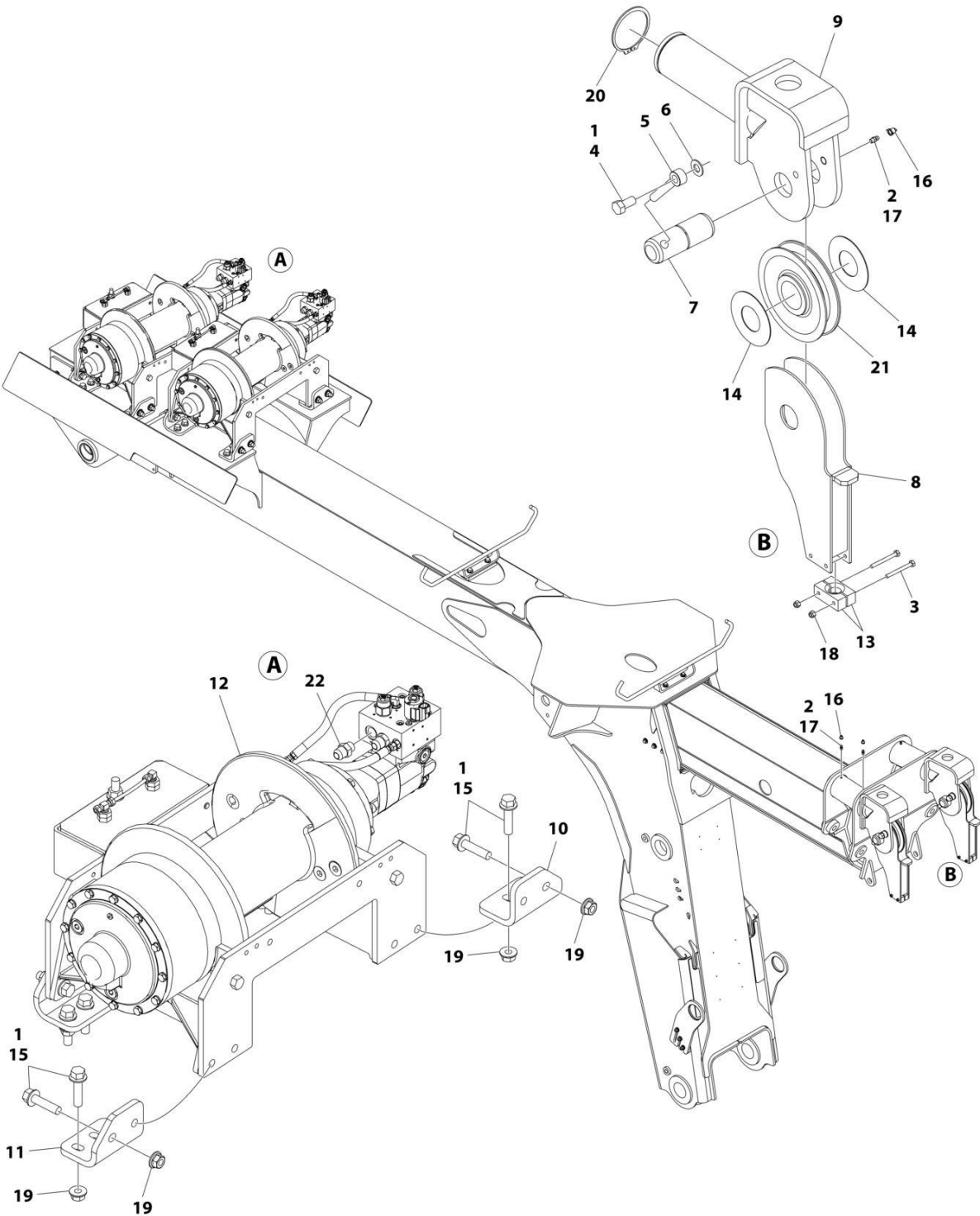
FIGURE 2-6. BOOM WINCH INSTALLATION - DP
