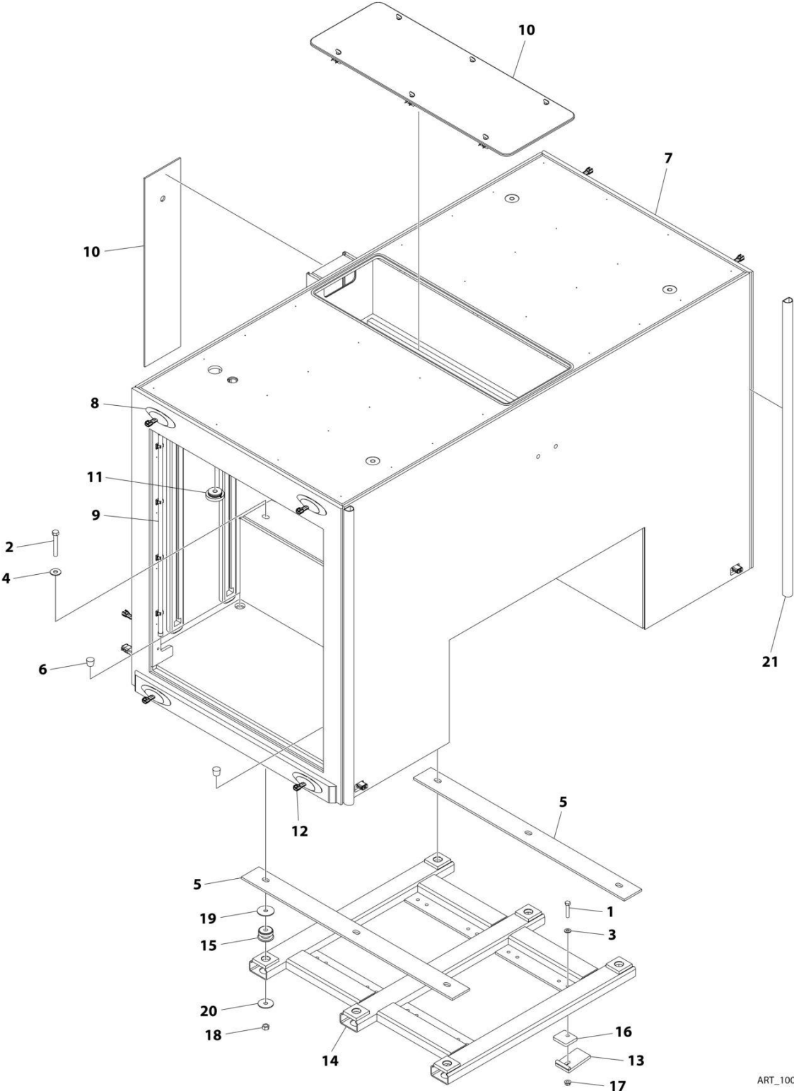
FIGURE 4-91. TUNNEL INSTALLATION (51IN WITH BATTERY)
