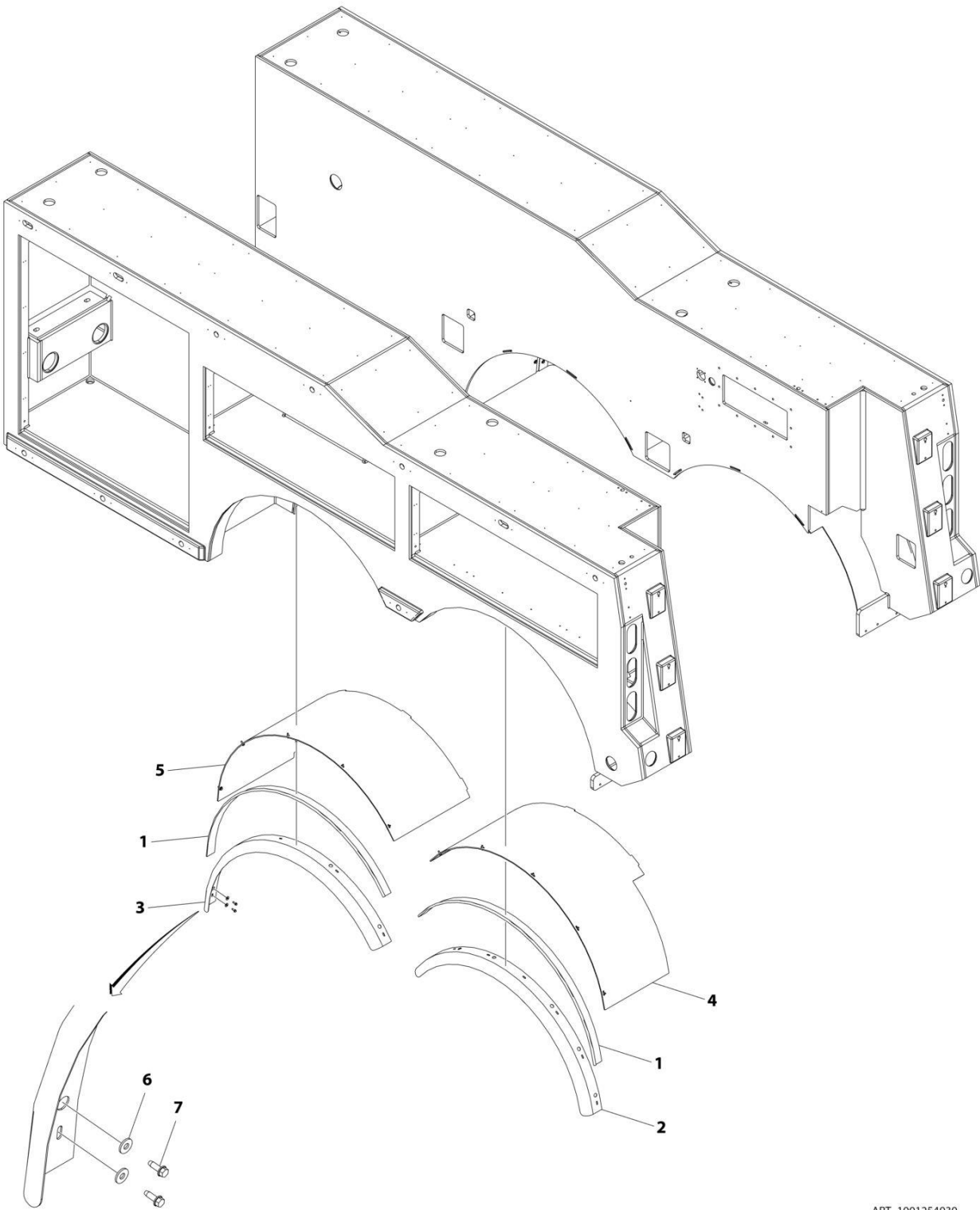
FIGURE 4-33. FENDER FLARE AND LINER INSTALLATION
