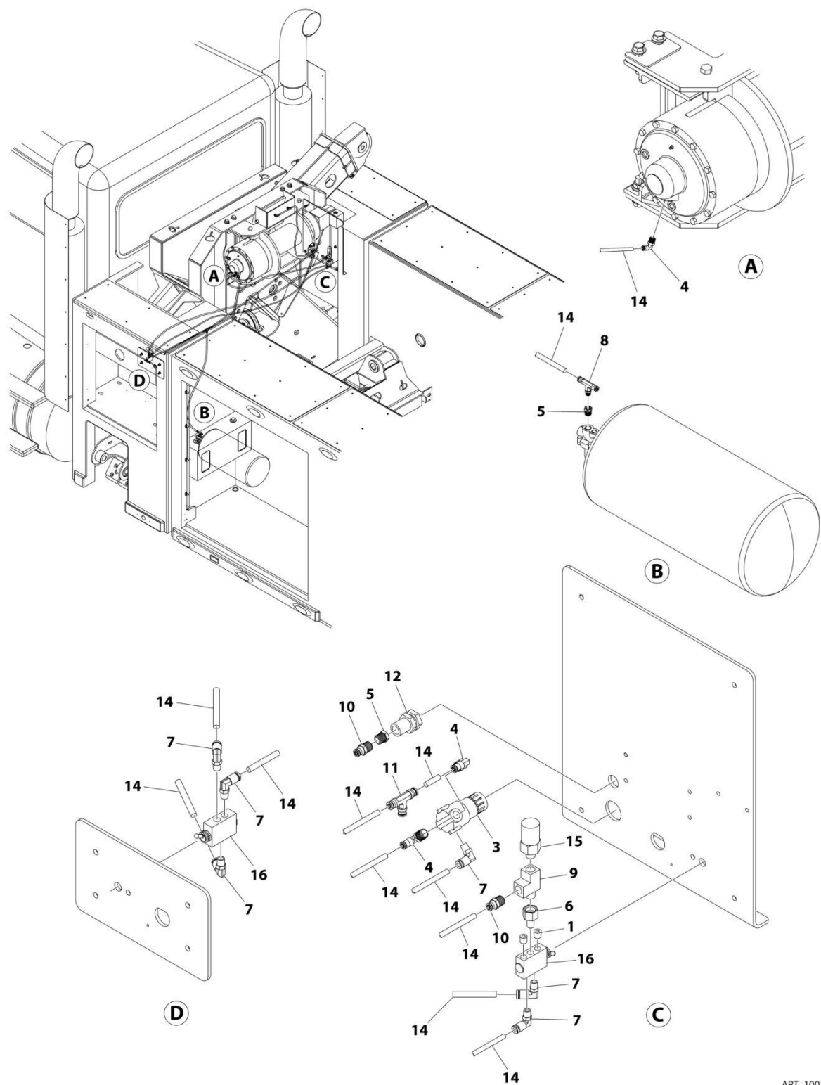
FIGURE 9-43. WINCH AIR INSTALLATION
