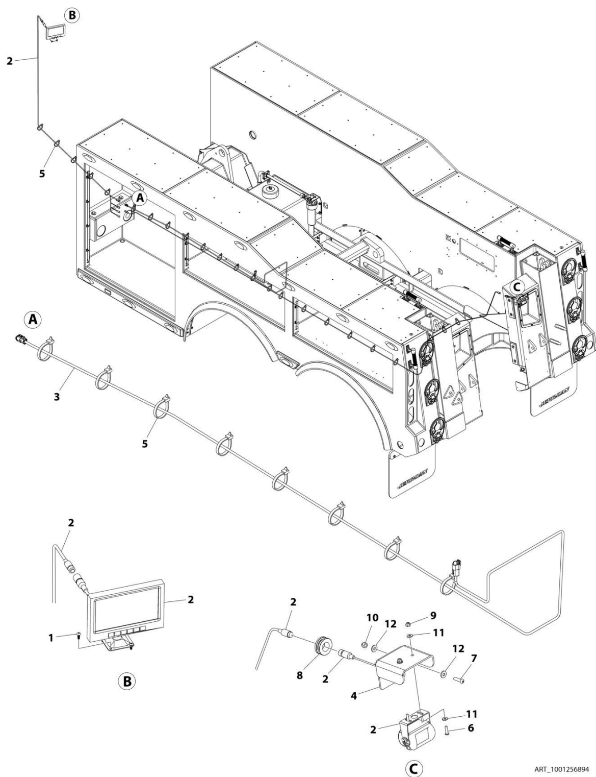
FIGURE 9-4. CAMERA INSTALLATION - BACK-UP (Prior to SN 0230009518)
