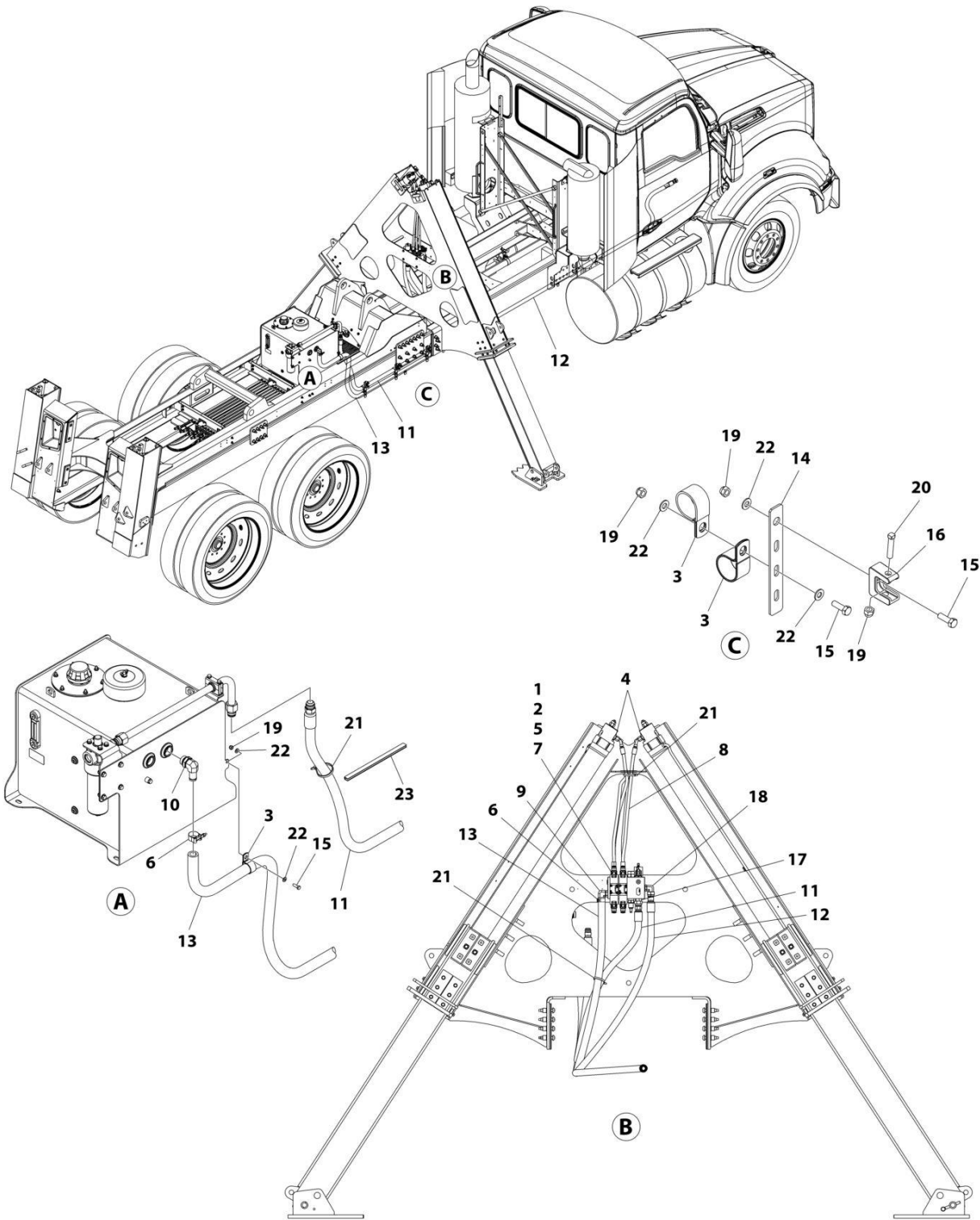
FIGURE 6-15. STABILIZER (SRS SS-70) HYDRAULIC INSTALLATION
