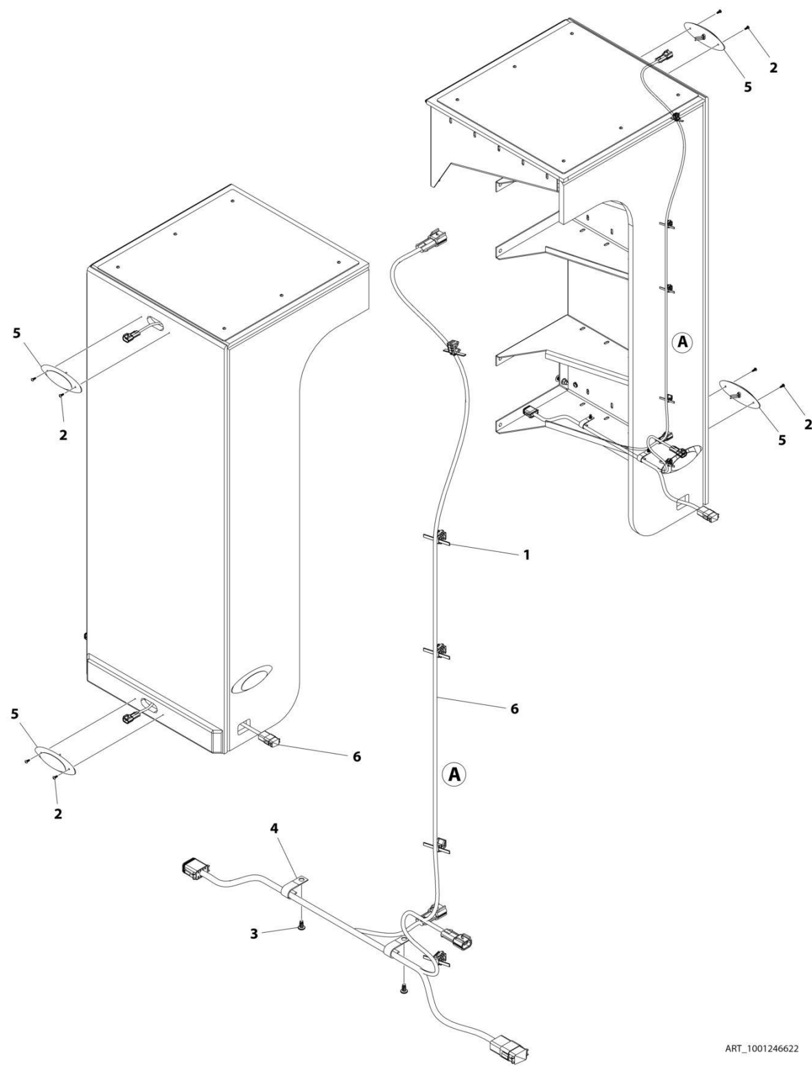
FIGURE 4-37. FILLER PANEL INSTALLATION - 24IN ELECTRICAL ENCLOSURE
