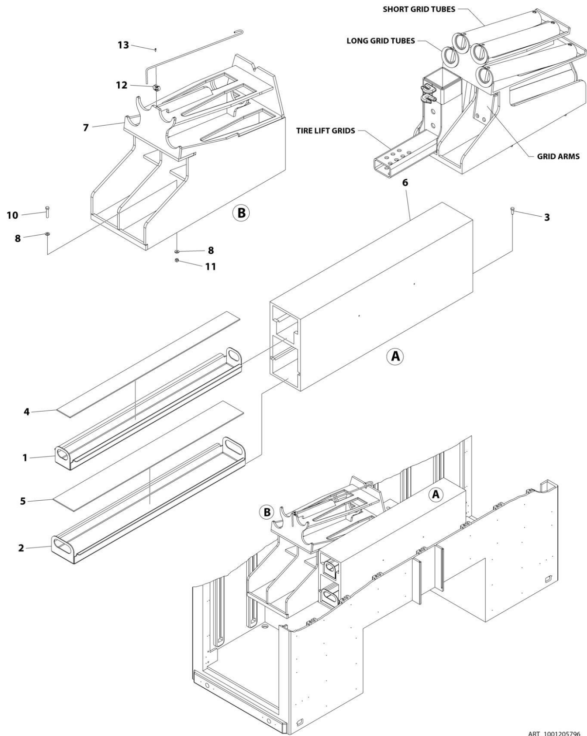
FIGURE 4-74. TIRE STORAGE INSTALLATION, 36IN
