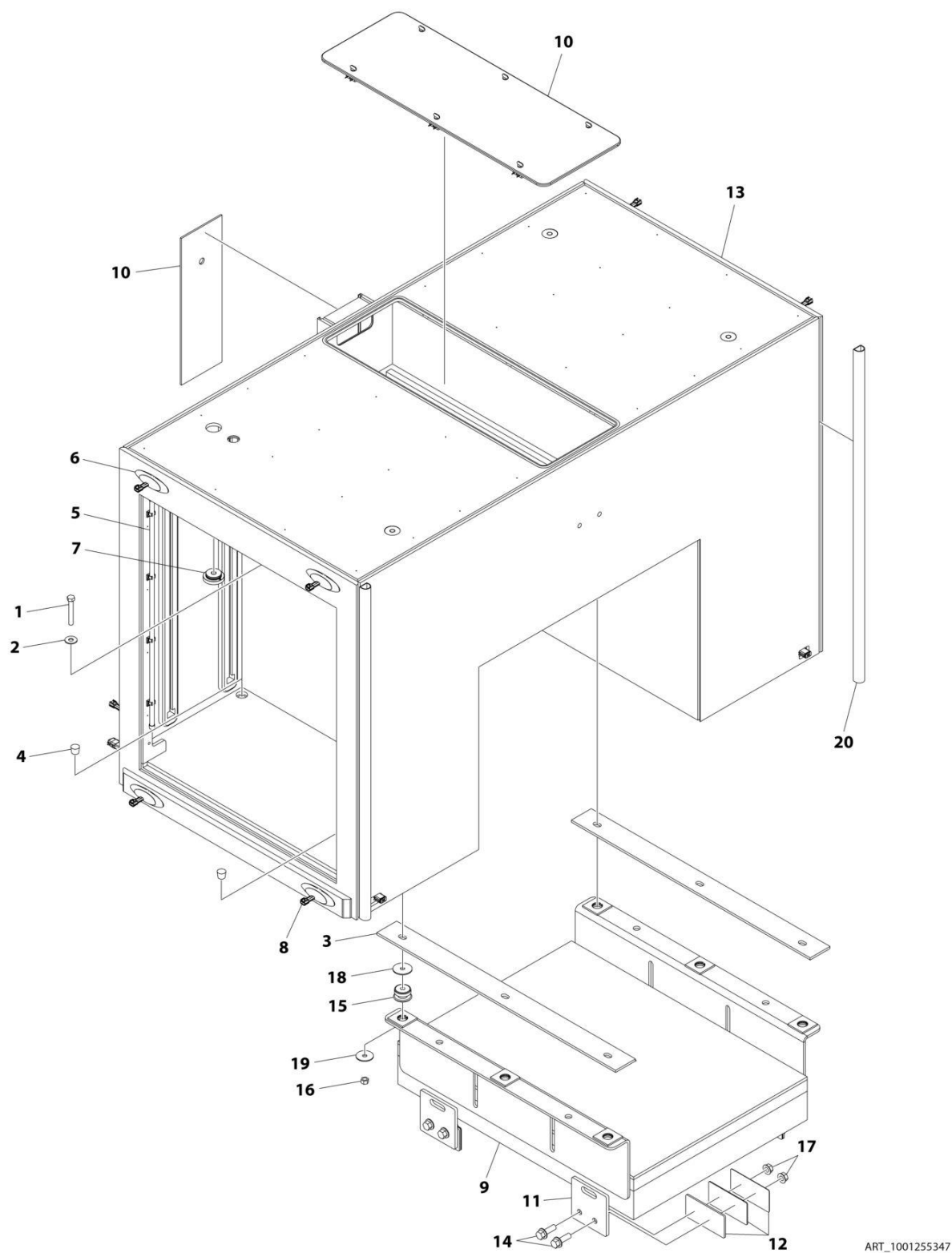
FIGURE 4-88. TUNNEL INSTALLATION (51IN TUNNEL WITH 3500 LBS COUNTERWEIGHT)
