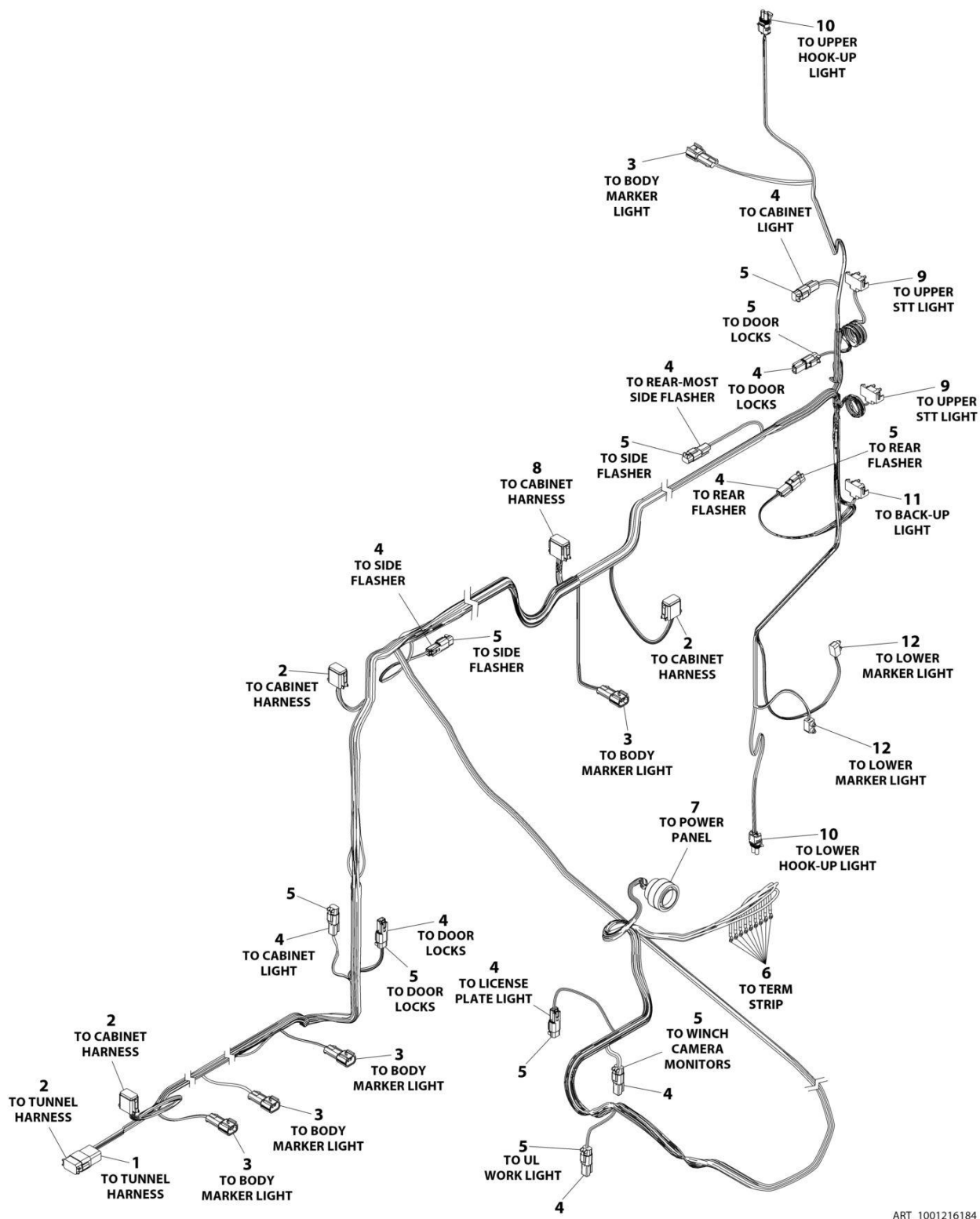
FIGURE 7-8. BODY HARNESS (RH)
