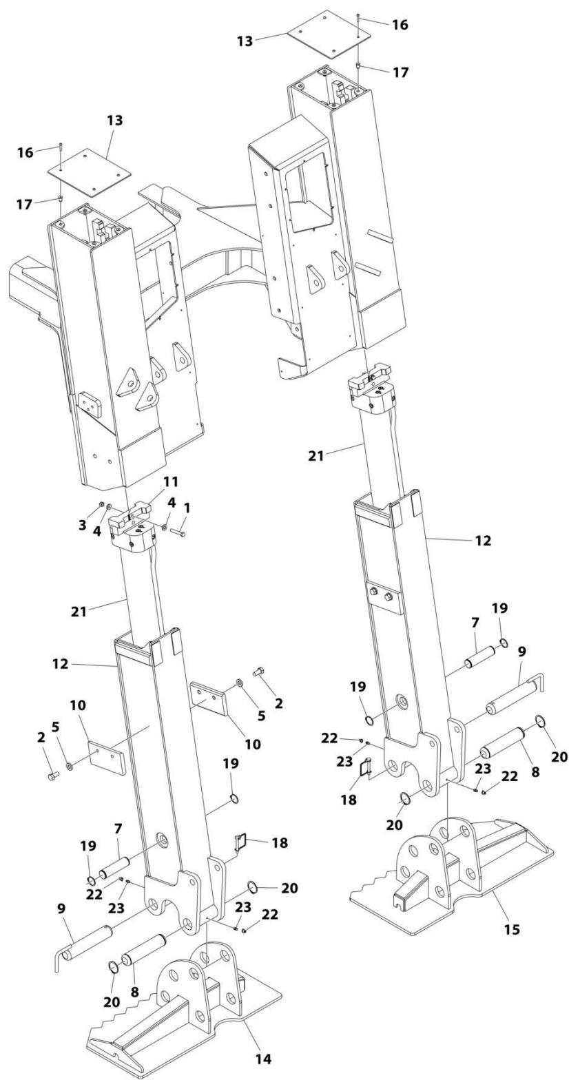
FIGURE 1-5. REAR STABILIZERS INSTALLATION (Prior to SN 0230007637)
