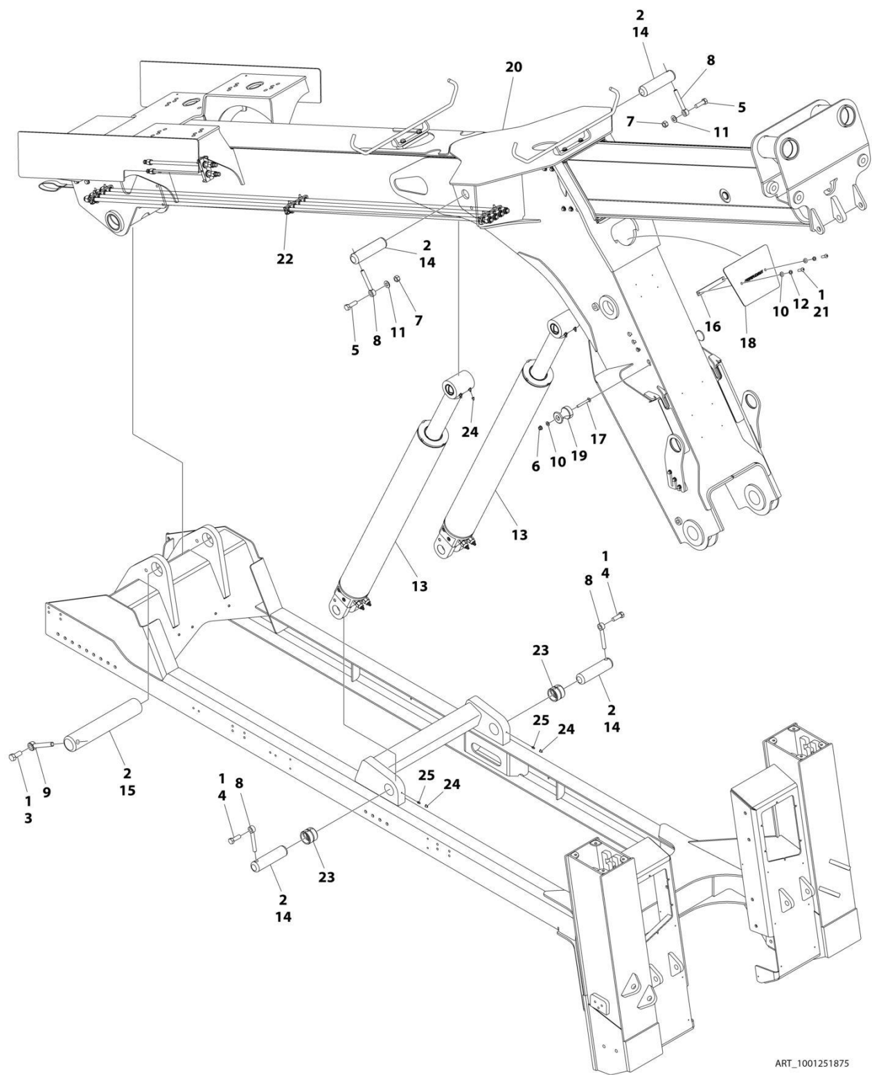
FIGURE 2-1. MAIN BOOM INSTALLATION (Prior to SN 0230007637)
