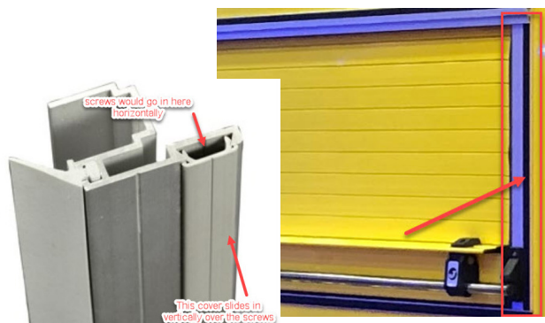
P SERIES SIDE RAIL FOR MODEL YEARS 2015 - MID-2025
